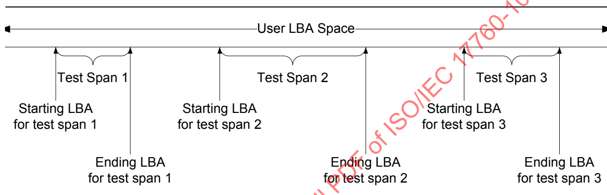
Figure 17 — Selective self-test span example
