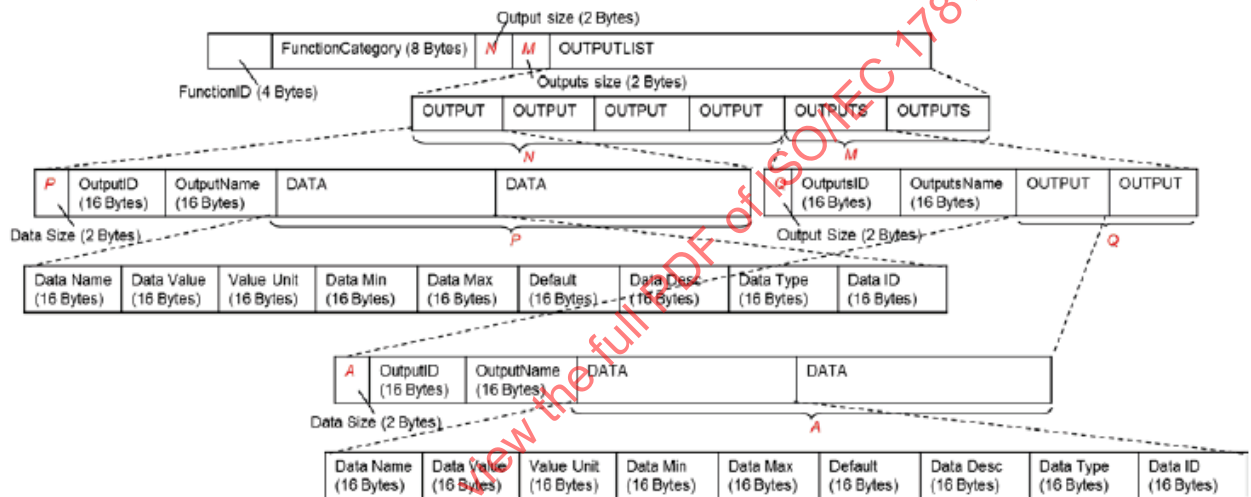
Figure 28 — DEVICE_CONTROL_RESPONSE Message Structure
