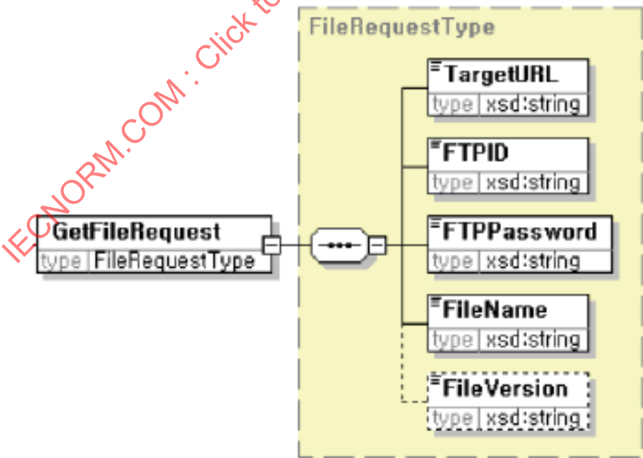
Figure C.22 — Get File Request Schema Structure
