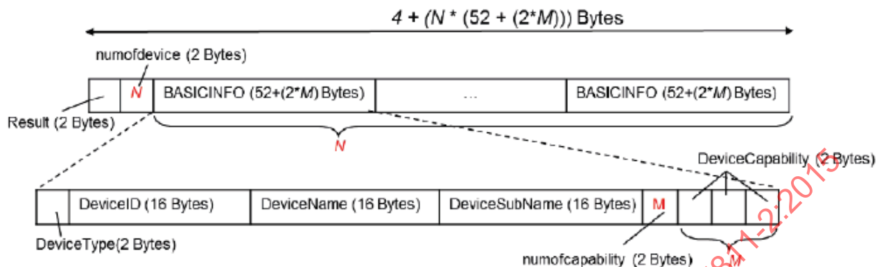
Figure 19 — DEVICE_INFO_RESPONSE Message Structure
