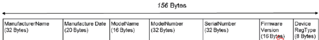
Figure 43 — DEVICE_REGISTRATION_REQUEST Message Structure
