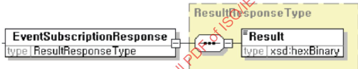
Figure C.19 — Event Subscription Response Schema Structure
