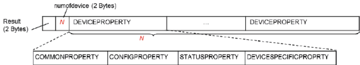
Figure 25 — DEVICE_INFO_RESPONSE Message Structure
