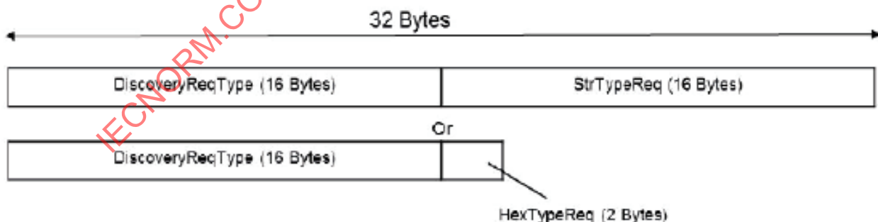
Figure 15 — DEVICE_DISCOVERY_REQUEST Message Structure
