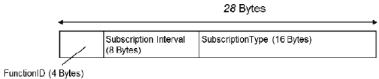
Figure 30 — EVENT_SUBSCRIPTION_REQUEST Message Structure
