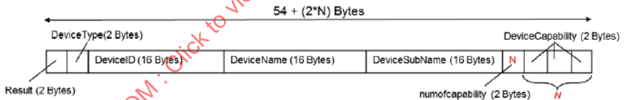
Figure 16 — DEVICE_DISCOVERY_RESPONSE Message Structure
