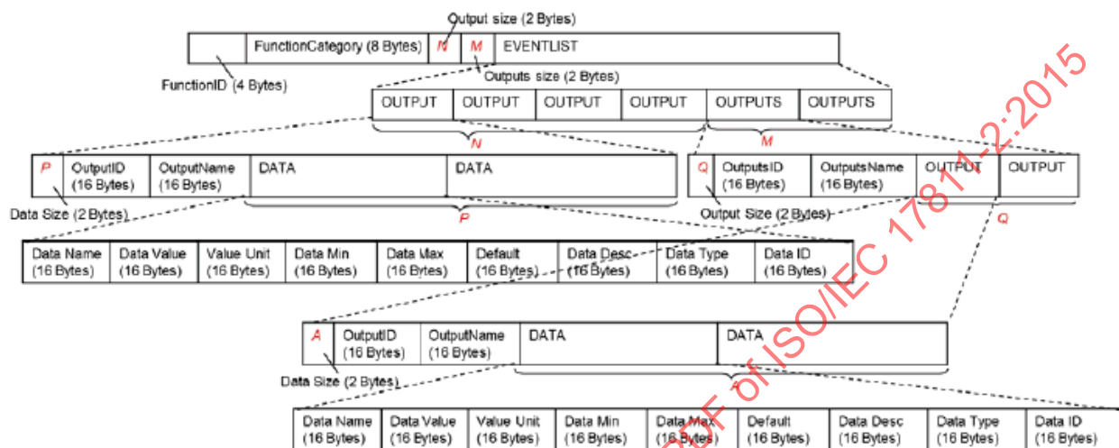
Figure 29 — EVENT_NOTIFICATION Message Structure
