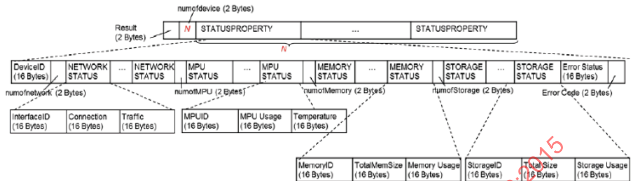
Figure 23 — DEVICE_INFO_RESPONSE Message Structure
