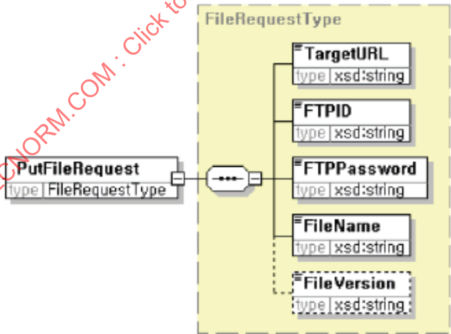
Figure C.25 — Put File Request Schema Structure
