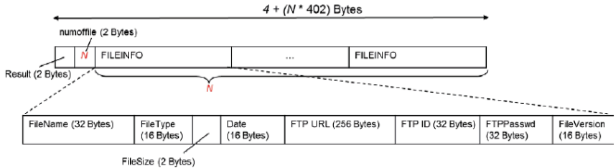
Figure 33 — GET_FILEINFO_RESPONSE Message Structure
