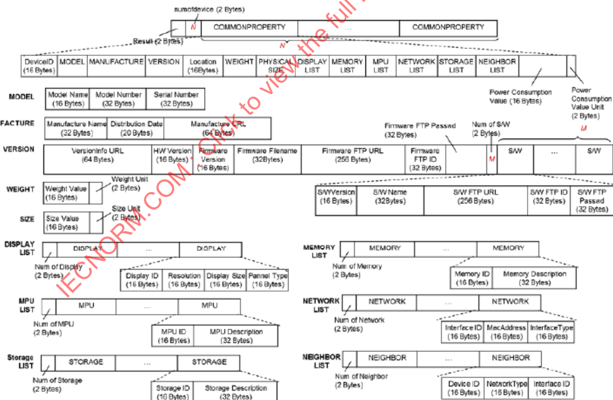
Figure 21 — DEVICE_INFO_RESPONSE Message Structure
