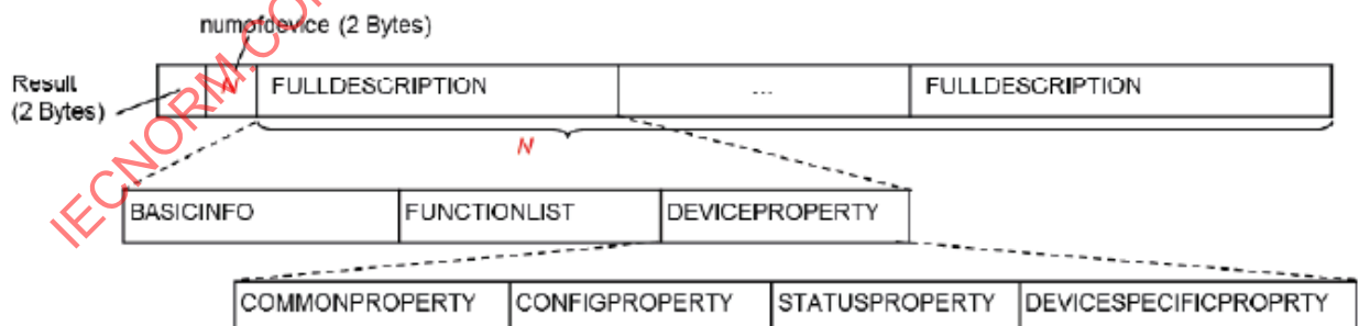
Figure 26 — DEVICE_INFO_RESPONSE Message Structure
