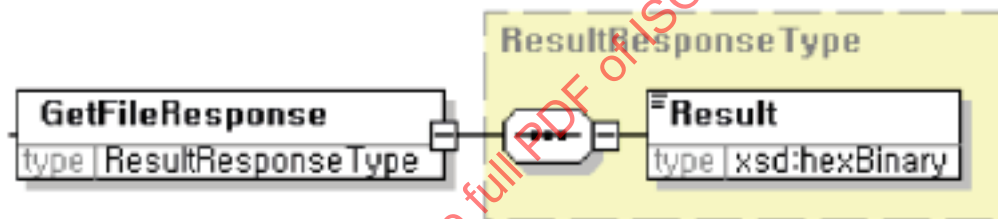
Figure C.23 — Get File Response Schema Structure
