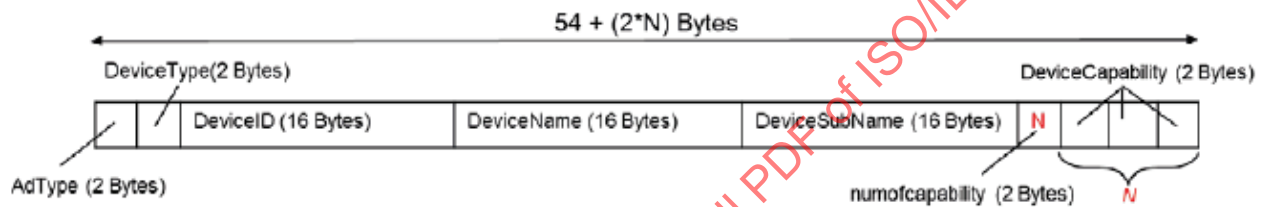
Figure 17 — DEVICE_ADVERTISEMENT Message Structure
