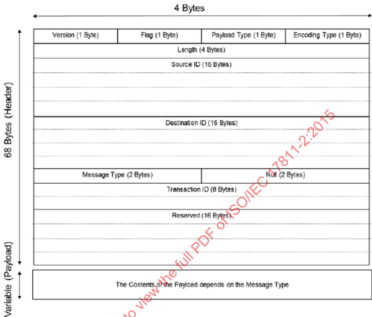
Figure 14 — DCMP Message Header Structure
