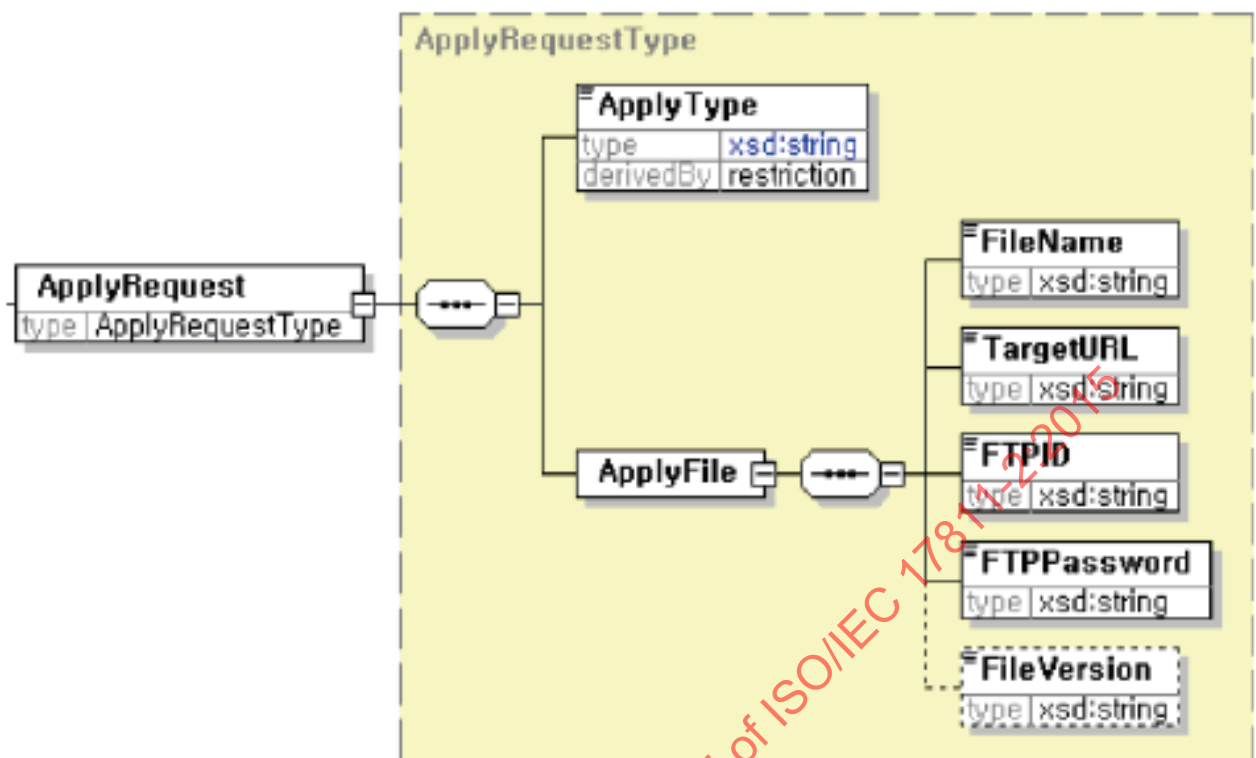
Figure C.28 — Apply Request Schema Structure
