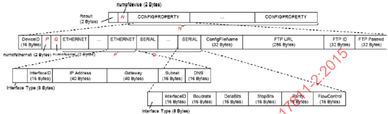
Figure 22 — DEVICE_INFO_RESPONSE Message Structure
