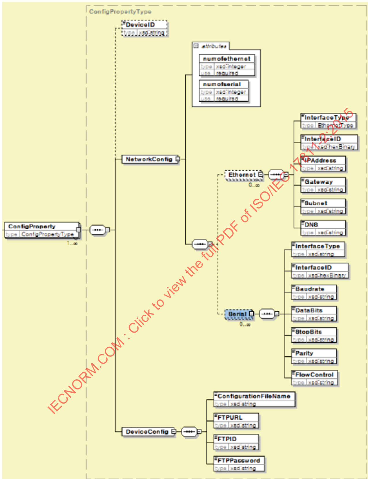
Figure C.12 — Config Property Message Schema Structure
