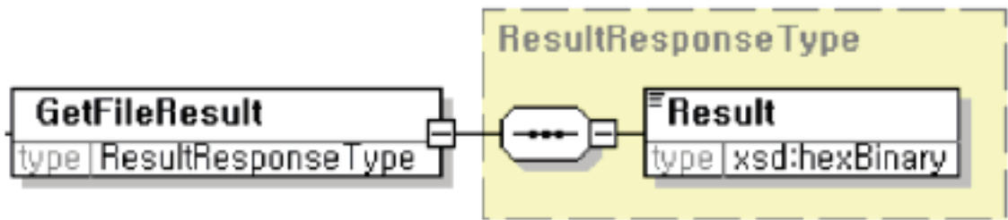
Figure C.24 — Get File Result Schema Structure
