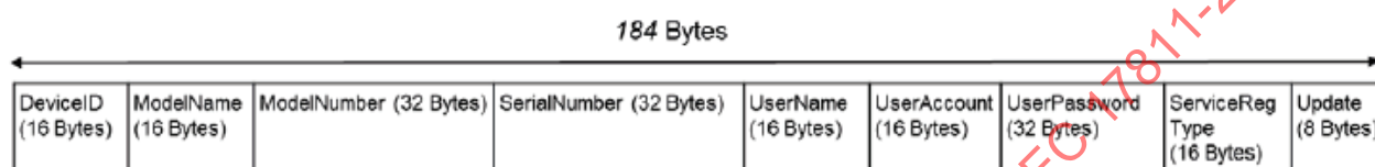
Figure 45 — SERVICE_REGISTRATION_REQUEST Message Structure
