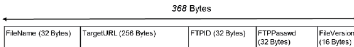
Figure 37 — PUT_FILE_REQUEST Message Structure
