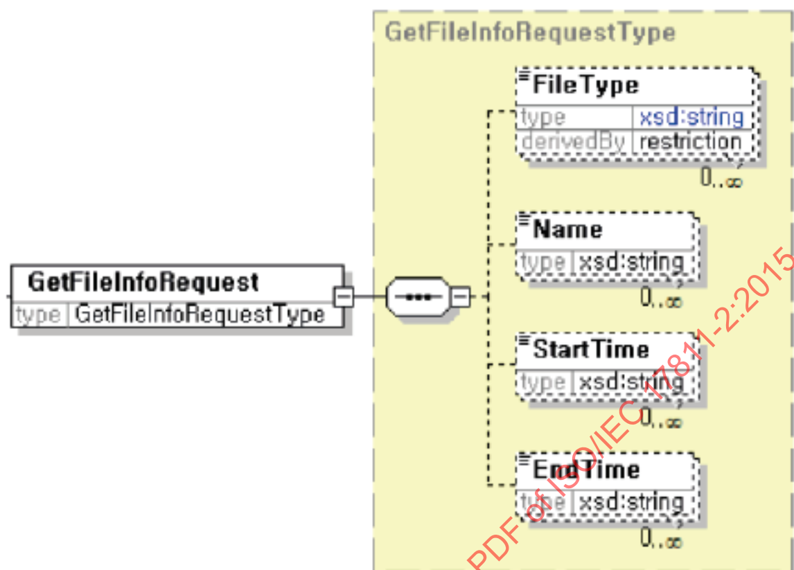
Figure C.20 — Get FileInfo Request Schema Structure
