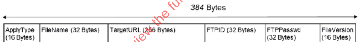
Figure 40 — APPLY_REQUEST Message Structure
