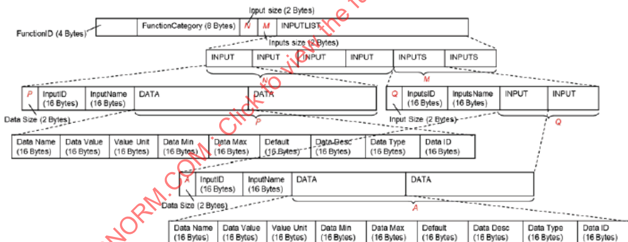
Figure 27 — DEVICE_CONTROL_REQUEST Message Structure
