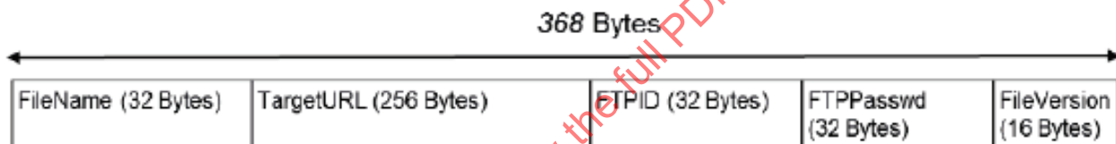
Figure 34 — GET_FILE_REQUEST Message Structure
