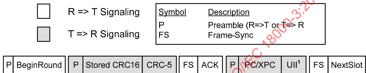
Figure 45 — One tag reply
