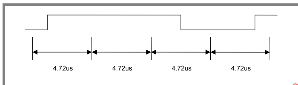
Figure 15 — 1 out of 4 mode example
