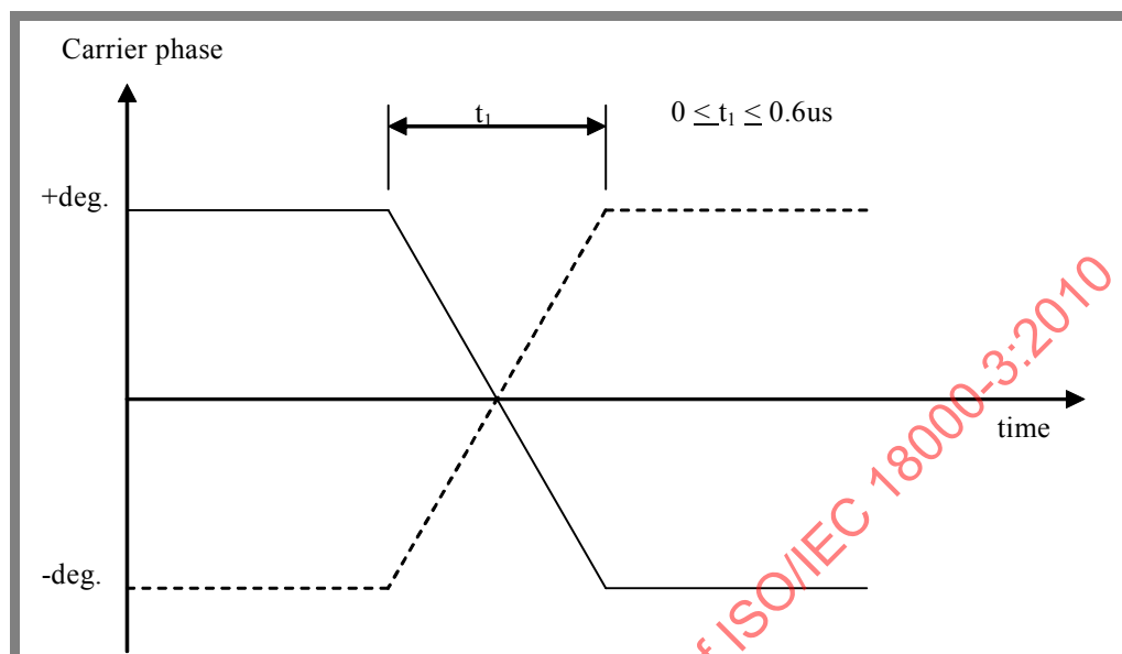
Figure 20 — PJM Method: Command modulation scheme
