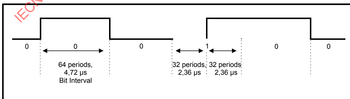
Figure 18 — PJM Method: Command MFM encoding and timing of binary 000100
