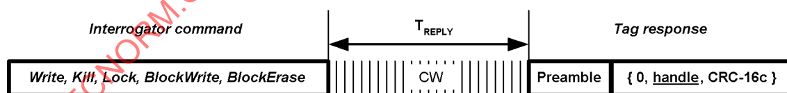
Figure 46 — Successful Write sequence
