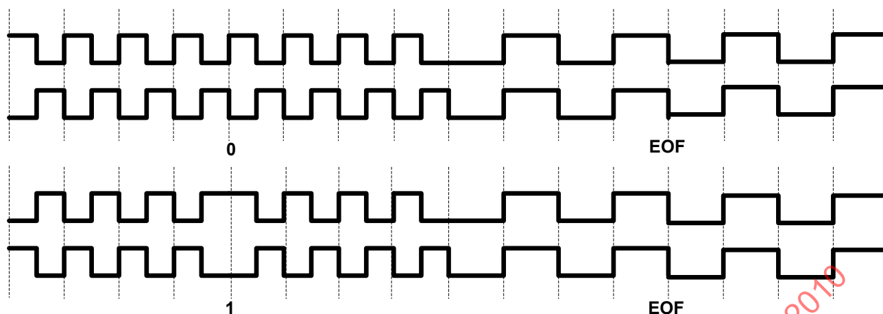
Figure 36 — ASK Method: Terminating subcarrier transmissions EOF
