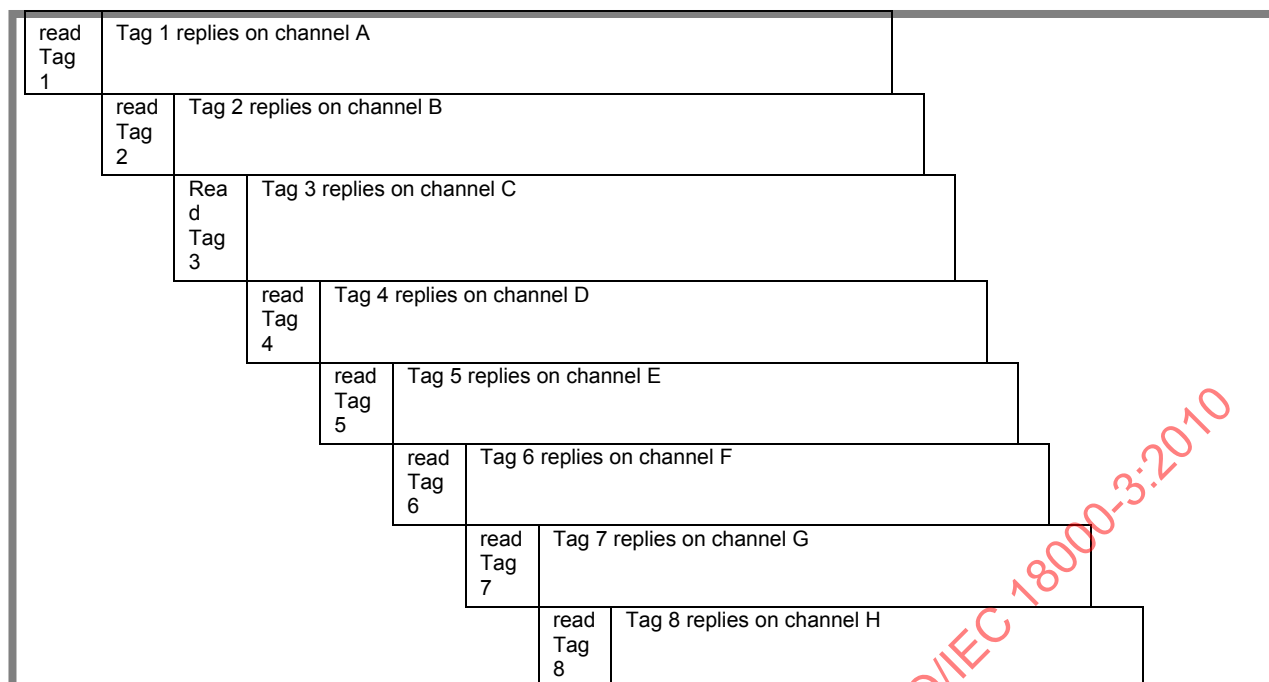
Figure 13 — Reading data from 8 tags
