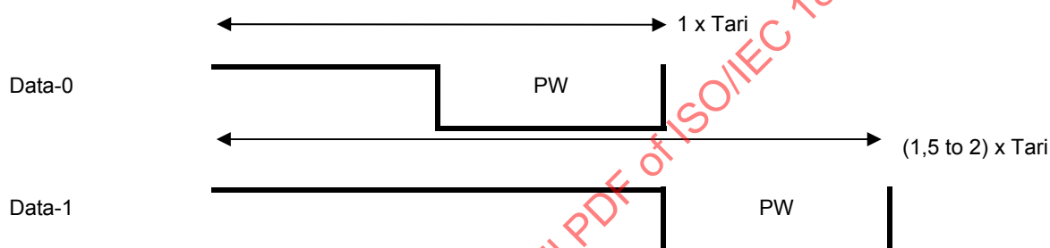
Figure 17 — ASK Method: PIE symbols
