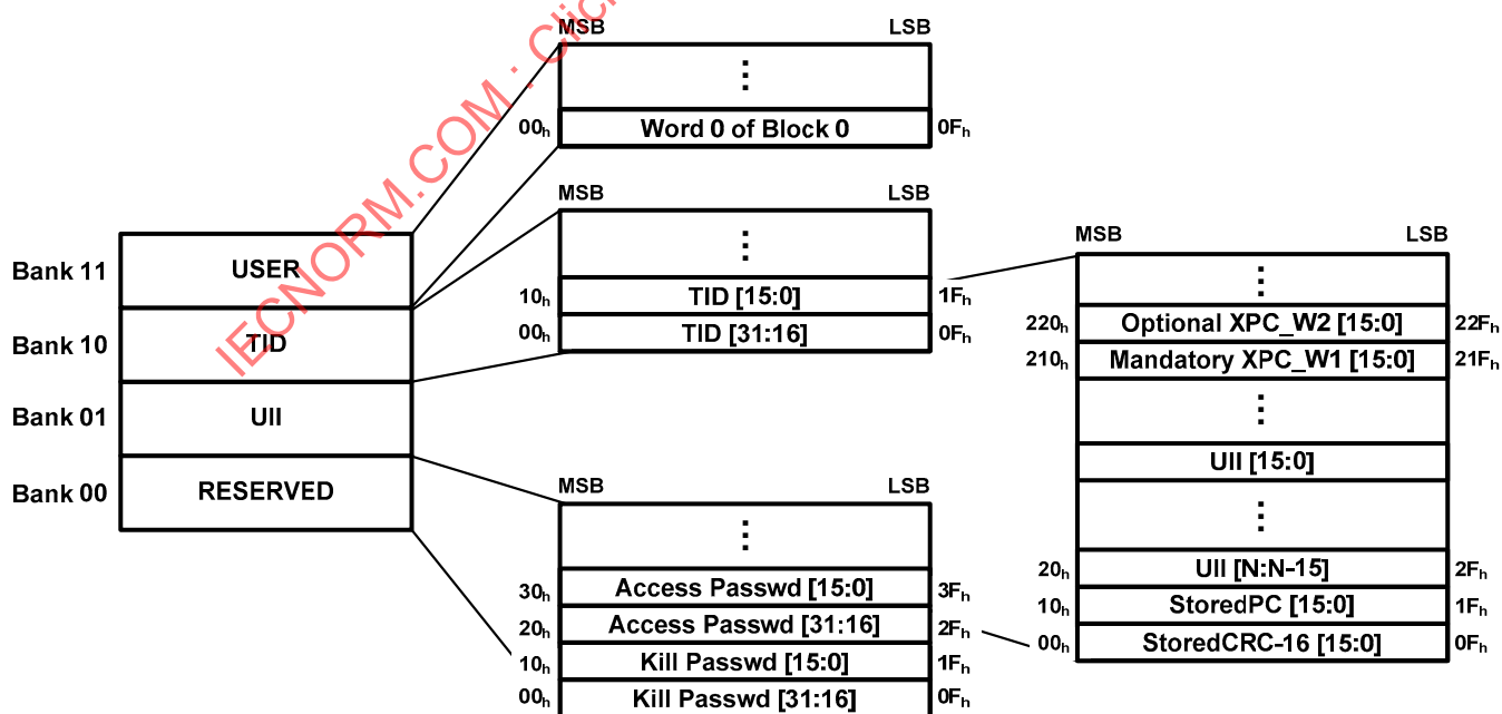
Figure 41 — Logical memory map
