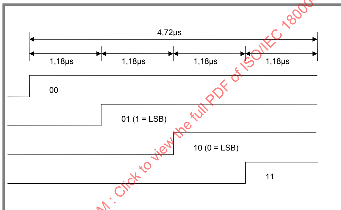
Figure 14 — 1 out of 4 mode encoding
