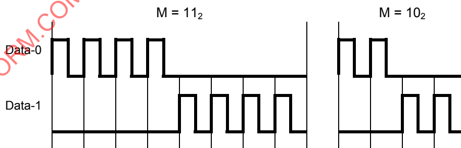
Figure 30 — ASK Method: Manchester subcarrier sequences
