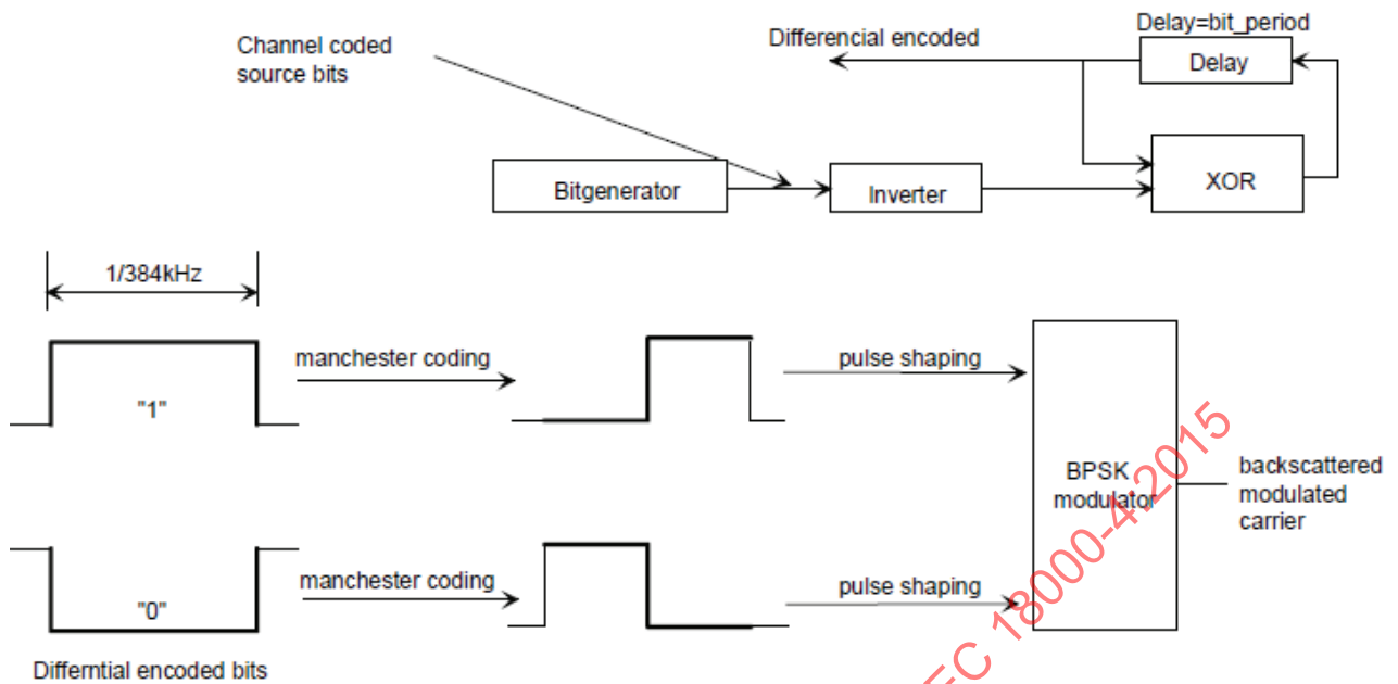
Figure 15 — Return link modulation and coding during communication
