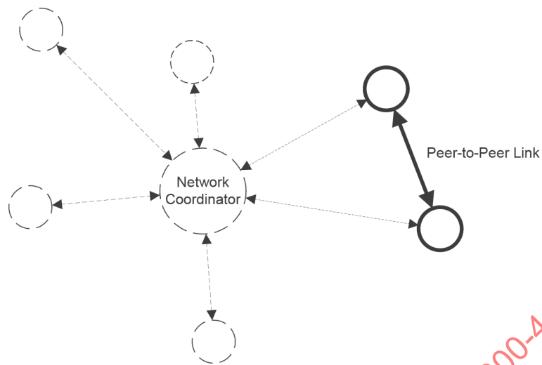
Figure 24 — Peer-to-Peer Topology
