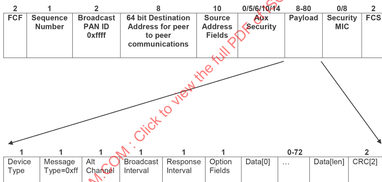
Figure 31 — Peer-to-Peer NDB Data Frame Description
