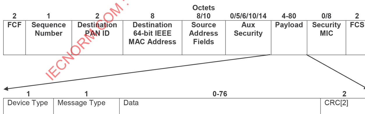
Figure 29 — General Description of Data Packet showing Payload Section
