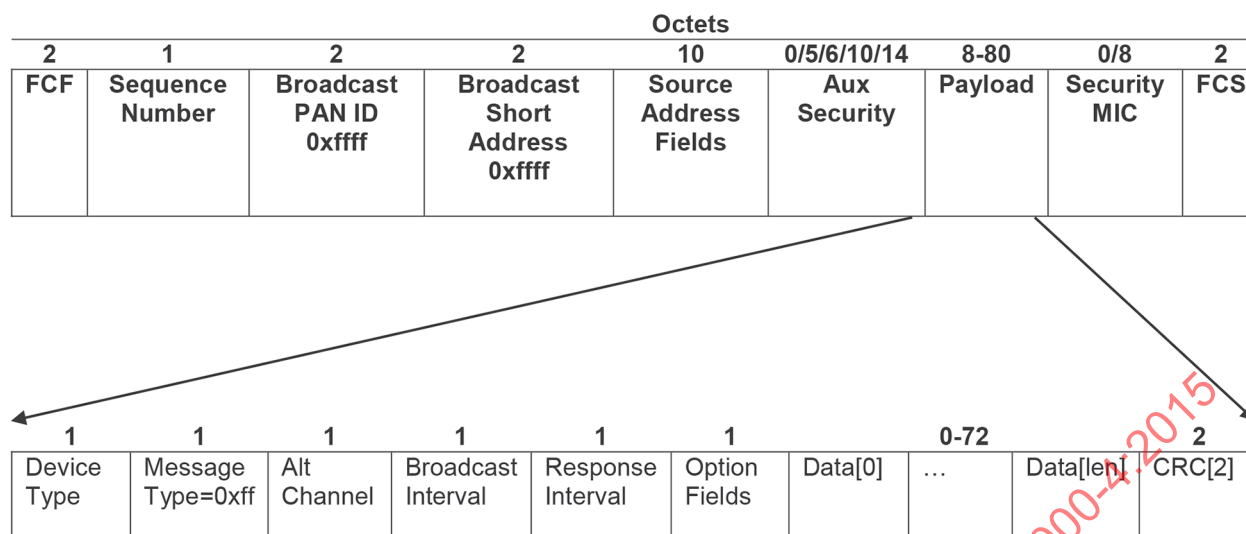
Figure 30 — Broadcast NDB Data Frame Description
