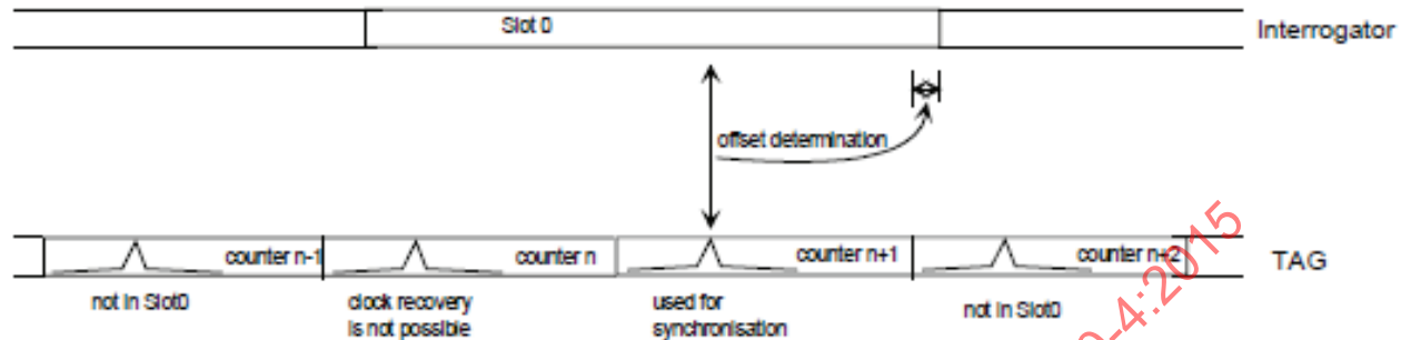
Figure 21 — S-CH position with regard to slot0
