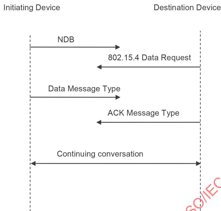
Figure 26 — Network Access for Peer to Peer Topology
