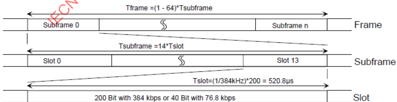
Figure 16 — Frame structure
