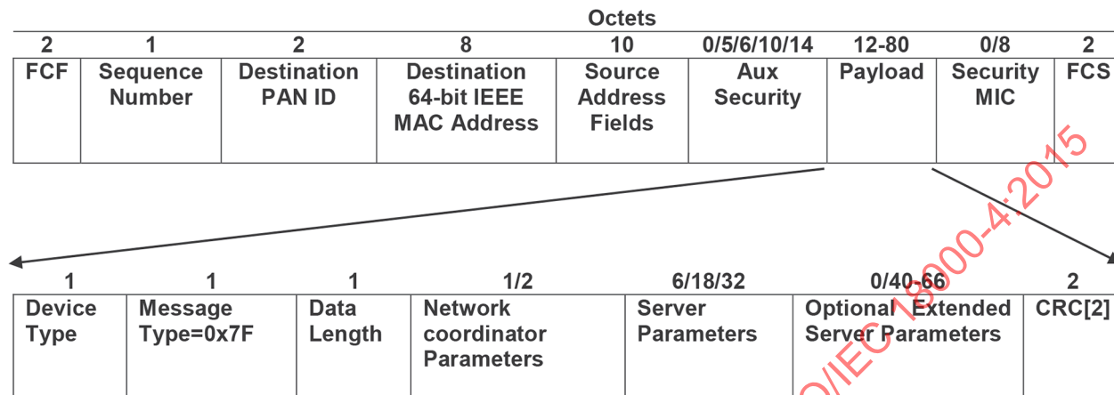
Figure 32 — Network Status Message Packet Description
