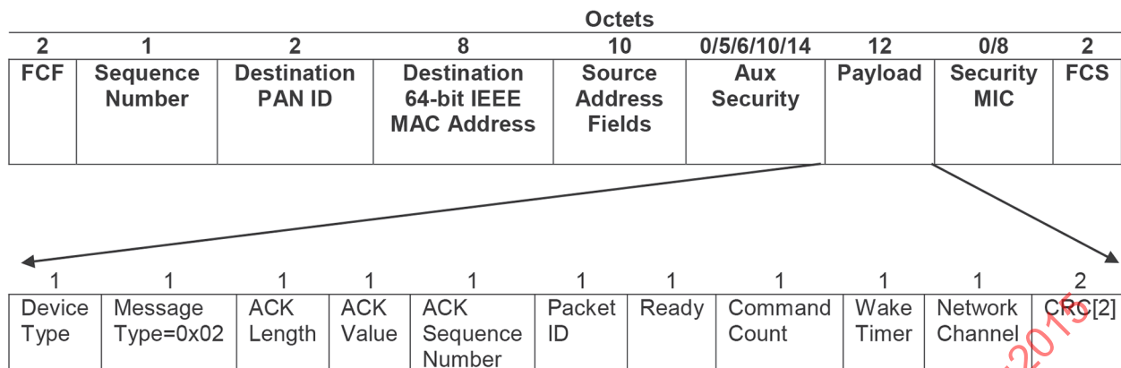
Figure 33 — Application ACK/NAK Packet Format
