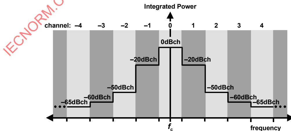
Figure Amd.1-9 — Transmit mask for multiple-interrogator environments
