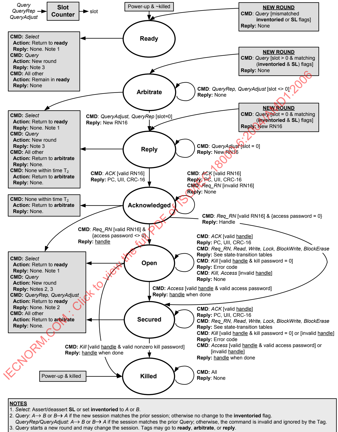
Figure Amd.1-22 — Tag state diagram
