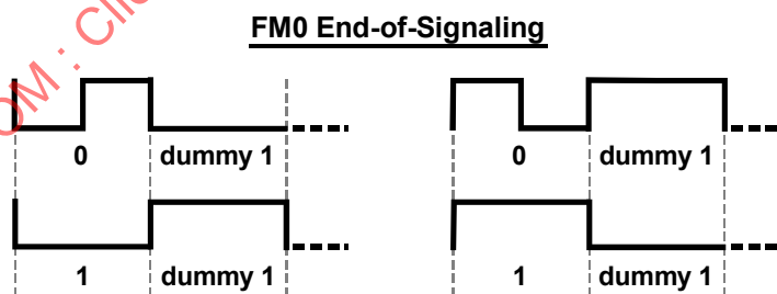
Figure Amd.1-13 — Terminating FM0 transmissions
