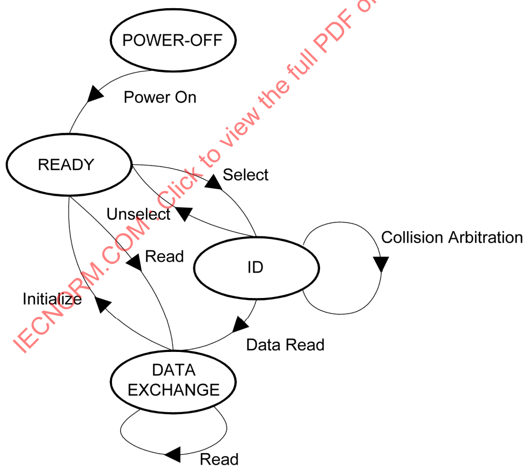
Figure 16 — State diagram
