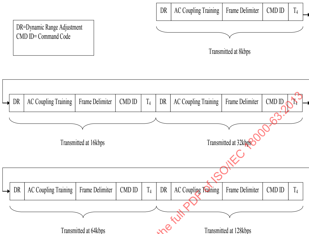
Figure 35 — Multirate_Reset command structure
