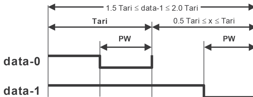
Figure 6.1 — PIE symbols
