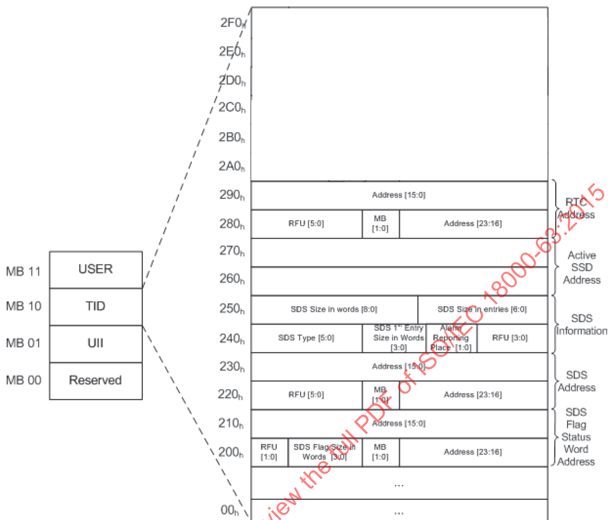
Figure 8.38 — Structure of TID memory
