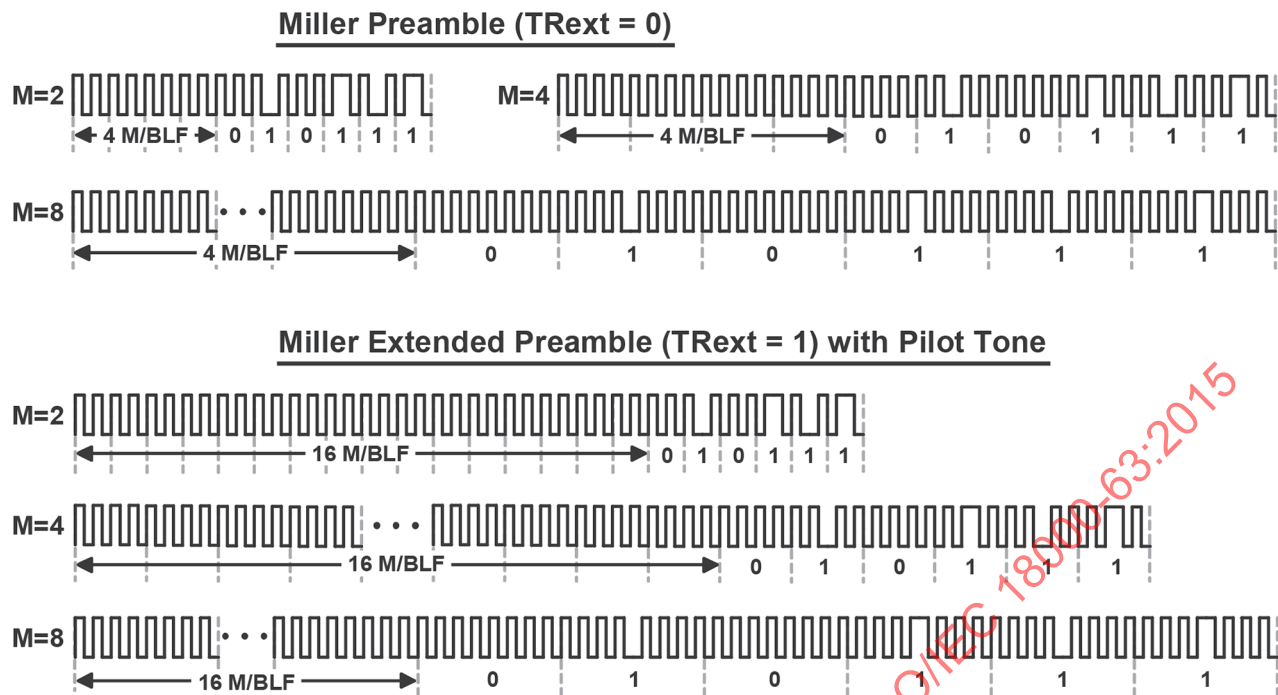
Figure 6.15 — Subcarrier T=&gt;R preamble
