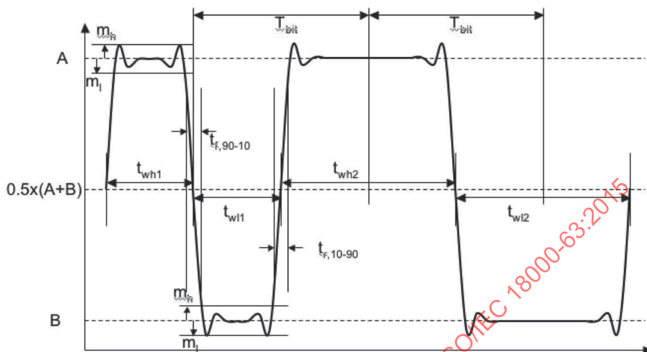
Figure 7.29 — Manchester waveform
