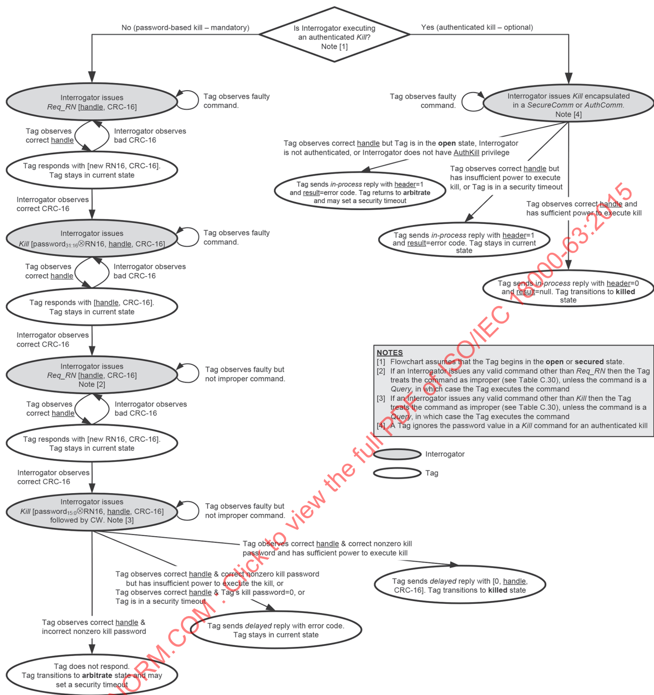
Figure 6.24 — Kill procedure
