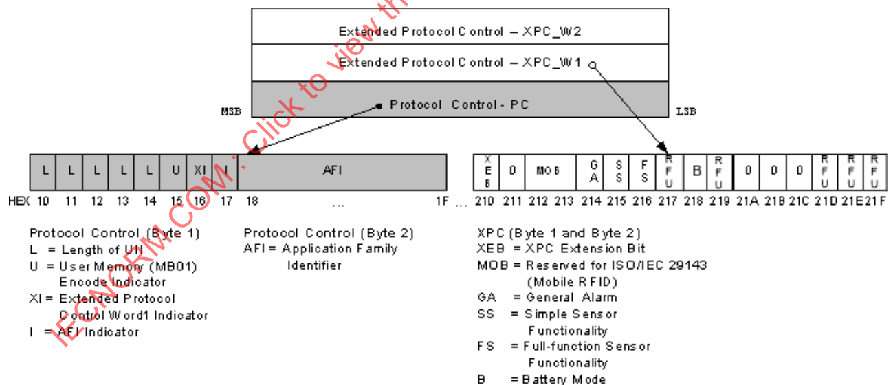
Figure 7.37 — Extended Protocol Control bit definitions (see NOTES 1 and 2)
