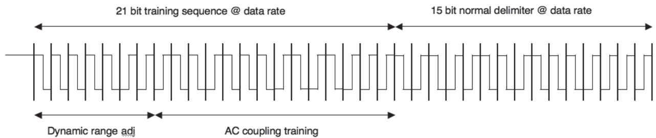
Figure 7.30 — Forward (R=>T) preamble
