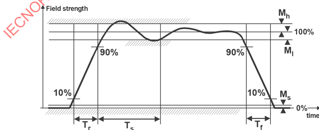
Figure 6.3 — Interrogator power-up and power-down RF envelope
