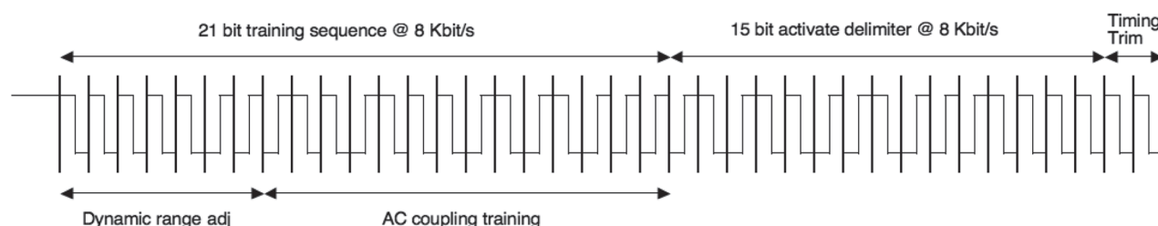
Figure 7.32 — Activation preamble
