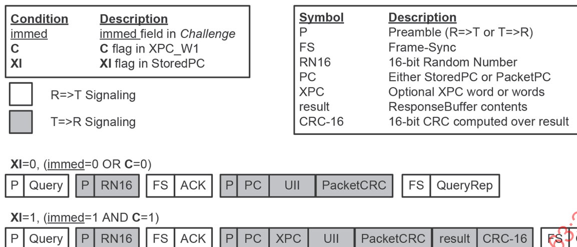
Figure 6.23 — One Tag reply
