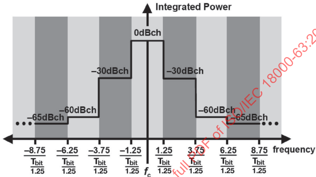
Figure 7.31 — Transmit mask for Manchester battery assisted mode
