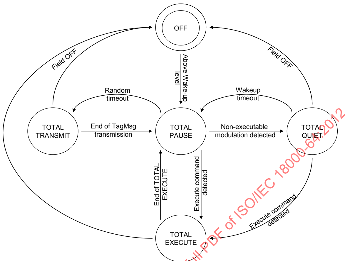
Figure 5 — TOTAL state diagram
