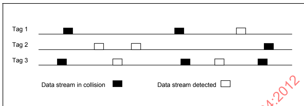
Figure 4 — Typical TOTAL Tag transmissions
