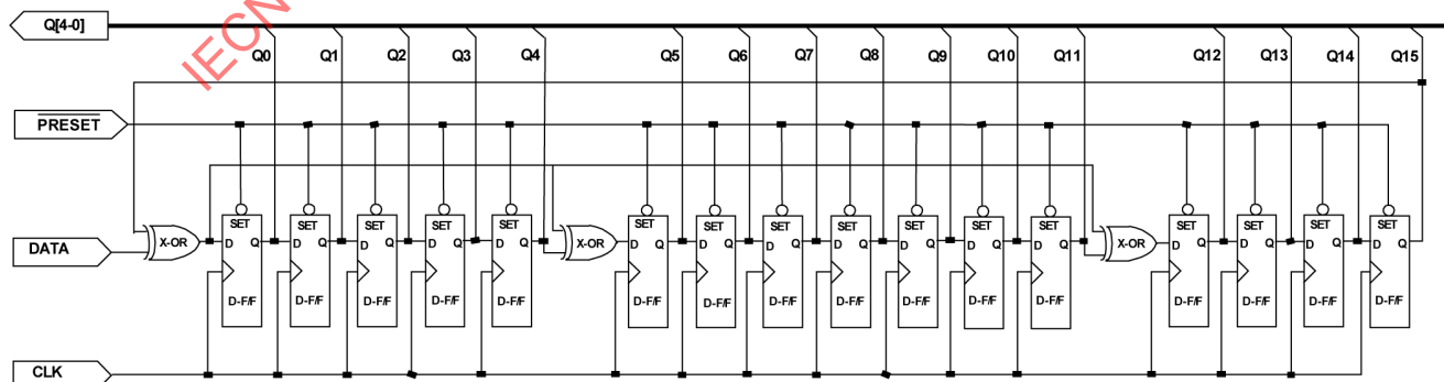
Figure A.2 — Example TID-S CRC-16 circuit
