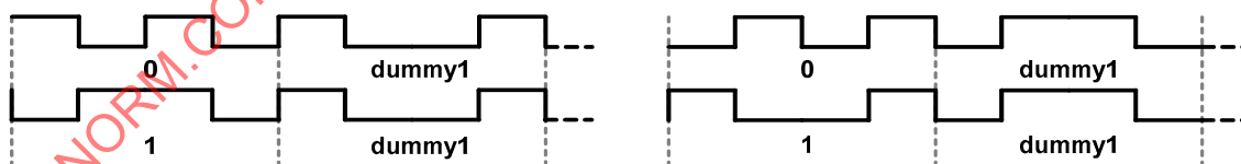
Figure 10 — Terminating Miller (M=2) subcarrier transmissions
