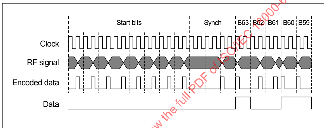
Figure 11 — PPE page modulation
