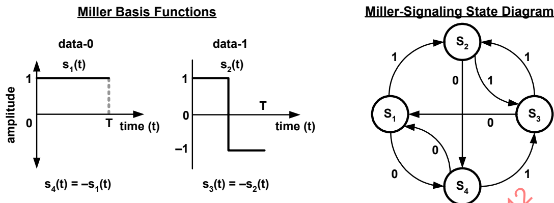
Figure 8 — Miller basis functions and generator state diagram
