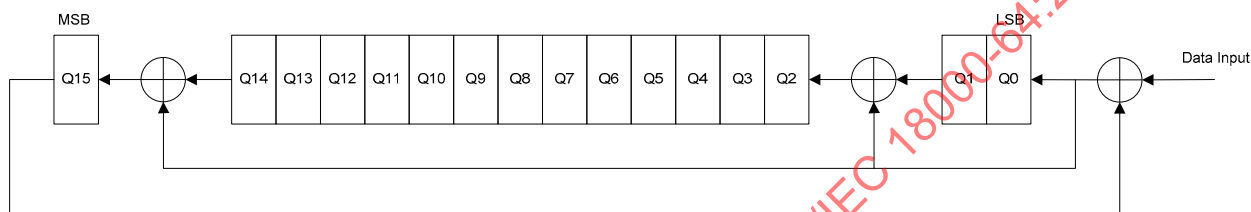
Figure A.3 — Example TID-U CRC-16 circuit
