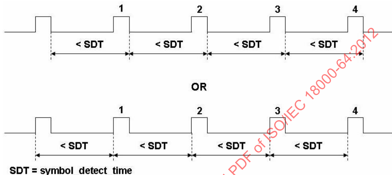
Figure 15 — Correct mute sequence
