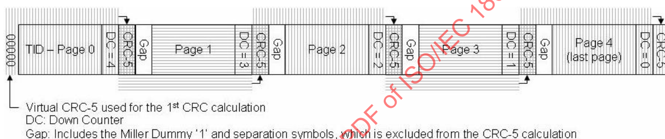
Figure 13 — Page link bits
