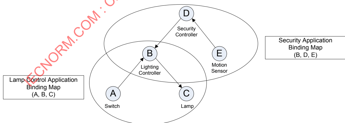
Figure 3 – Binding map example
