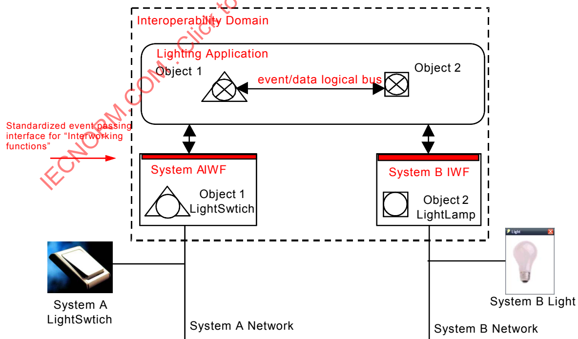
Figure A.1 – Lighting application of logical components
