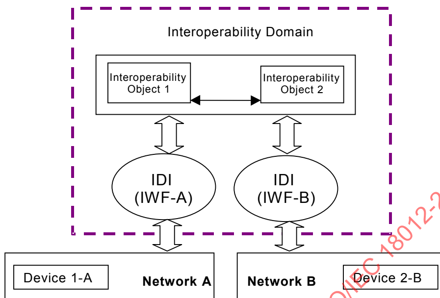
Figure 2 – Application interoperability model
