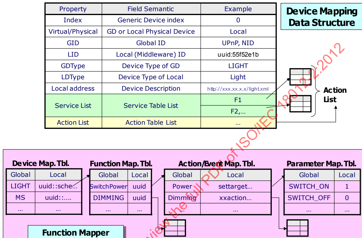
Figure A.10 – System B function mapping table
