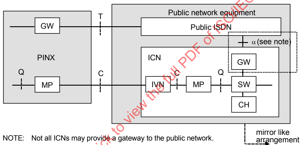
Figure 3 - VPN access with separate interfaces for public and PISN calls
