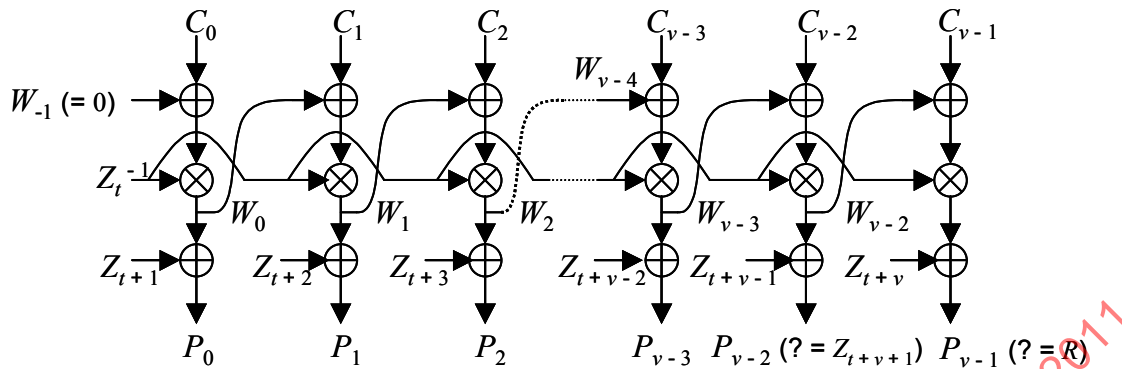
Figure 2 — Out^{-1} function of MULTI-S01 mode
