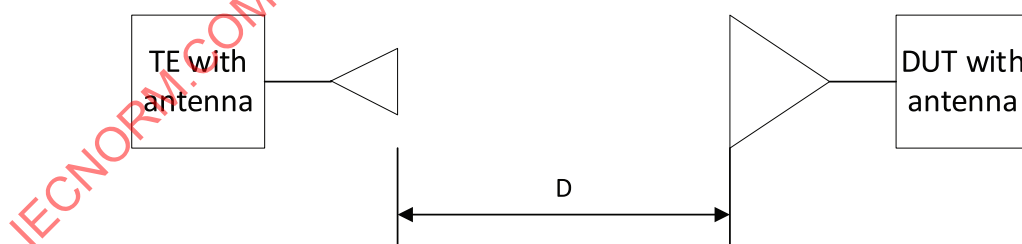
Figure 3 — Contactless test setup
