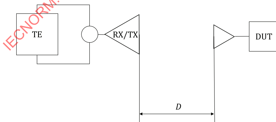
Figure 2 — Monostatic test setup
