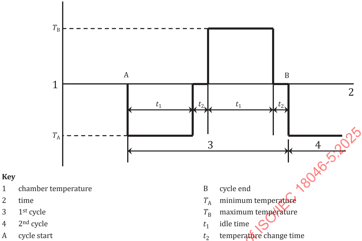
Figure 2 — Temperature change test cycle configuration
