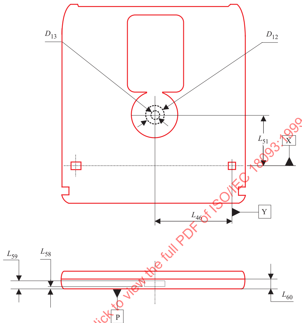
Figure 13 - Capture cylinder
