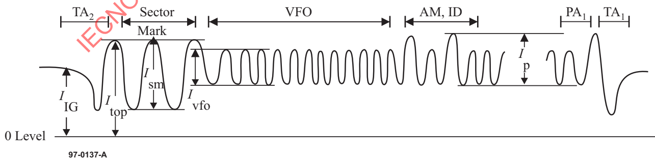
Figure 23c - Signals from Headers in Channel 1
