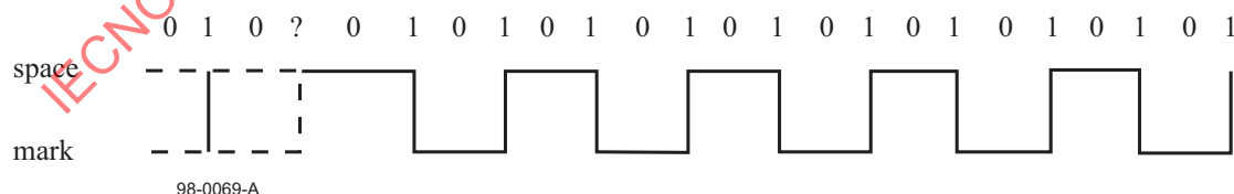
Figure 18 - Postamble pattern
