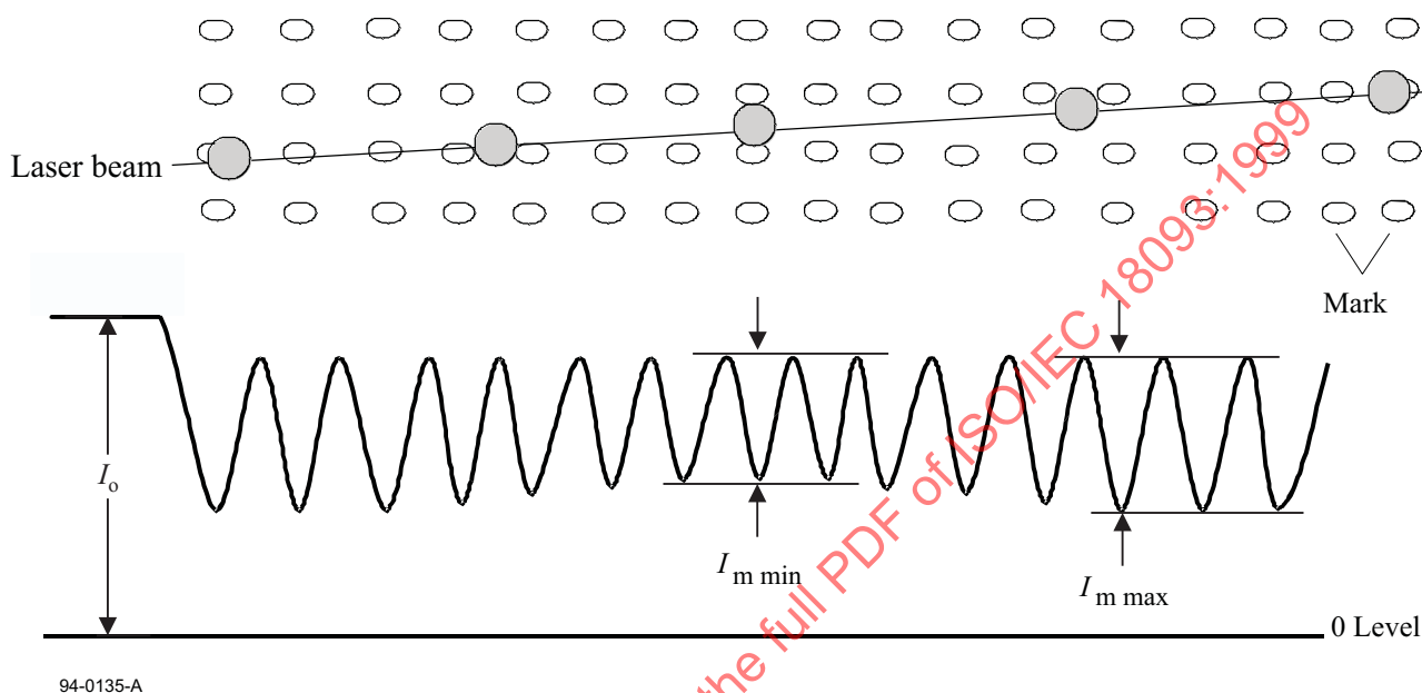
Figure 24 - Path of the laser beam when crossing tracks and the resulting PEP signals
