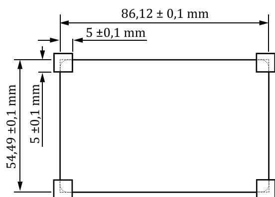
Figure D.5 — ICC holding geometry with ICC (top view and 3D view)
