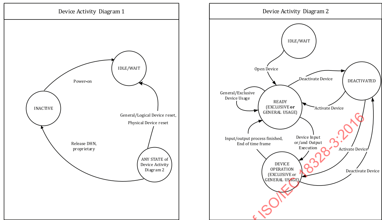
Figure 2 — State diagram of electronic device activities
