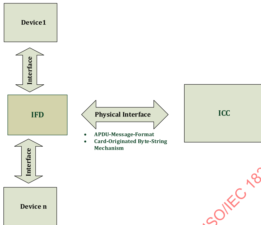
Figure 4 — System architecture for usage of off-card devices
