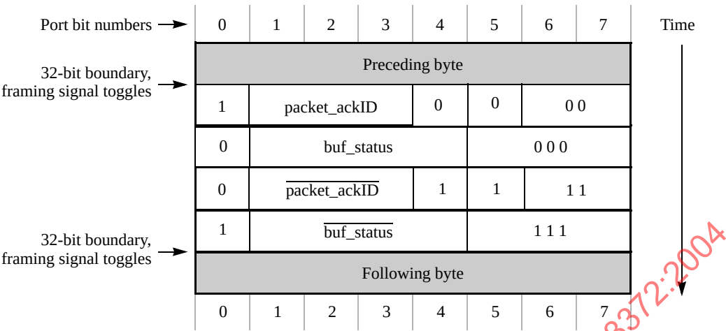
Figure 3-7. Control Symbol Transmission Example 1
