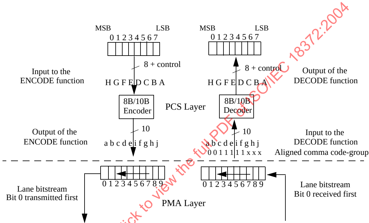
Figure 4-3. Lane Encoding, Serialization, Deserialization, and Decoding Process
