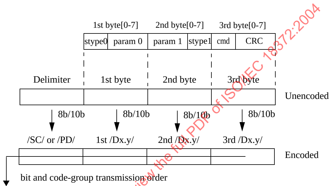
Figure 4-5. 1x Mode Control Symbol Encoding and Transmission Order
