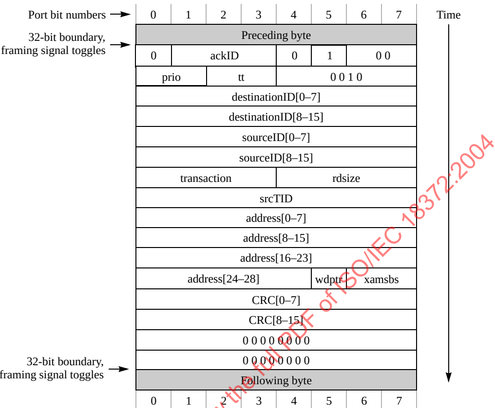
Figure 2-12. Request Packet Transmission Example 3
