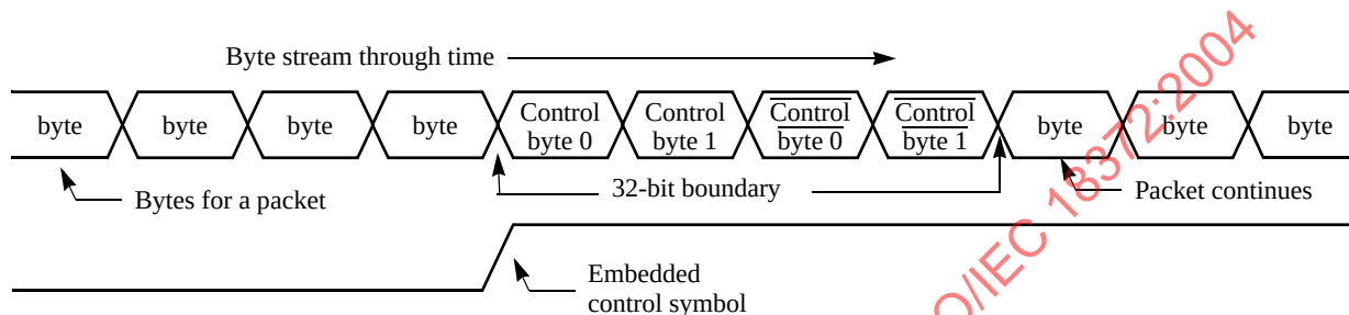
Figure 2-8. Embedded Control Symbols for 8-bit Port
