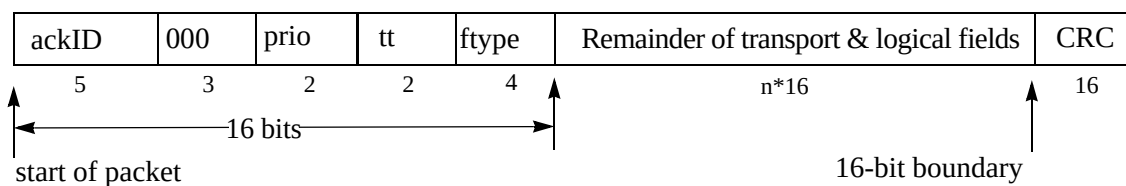
Figure 2-2. Packet Alignment
