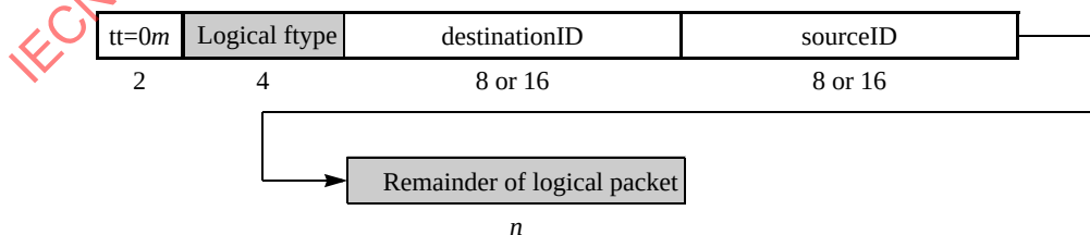
Figure 1-3. Destination-Source Transport Bit Stream
