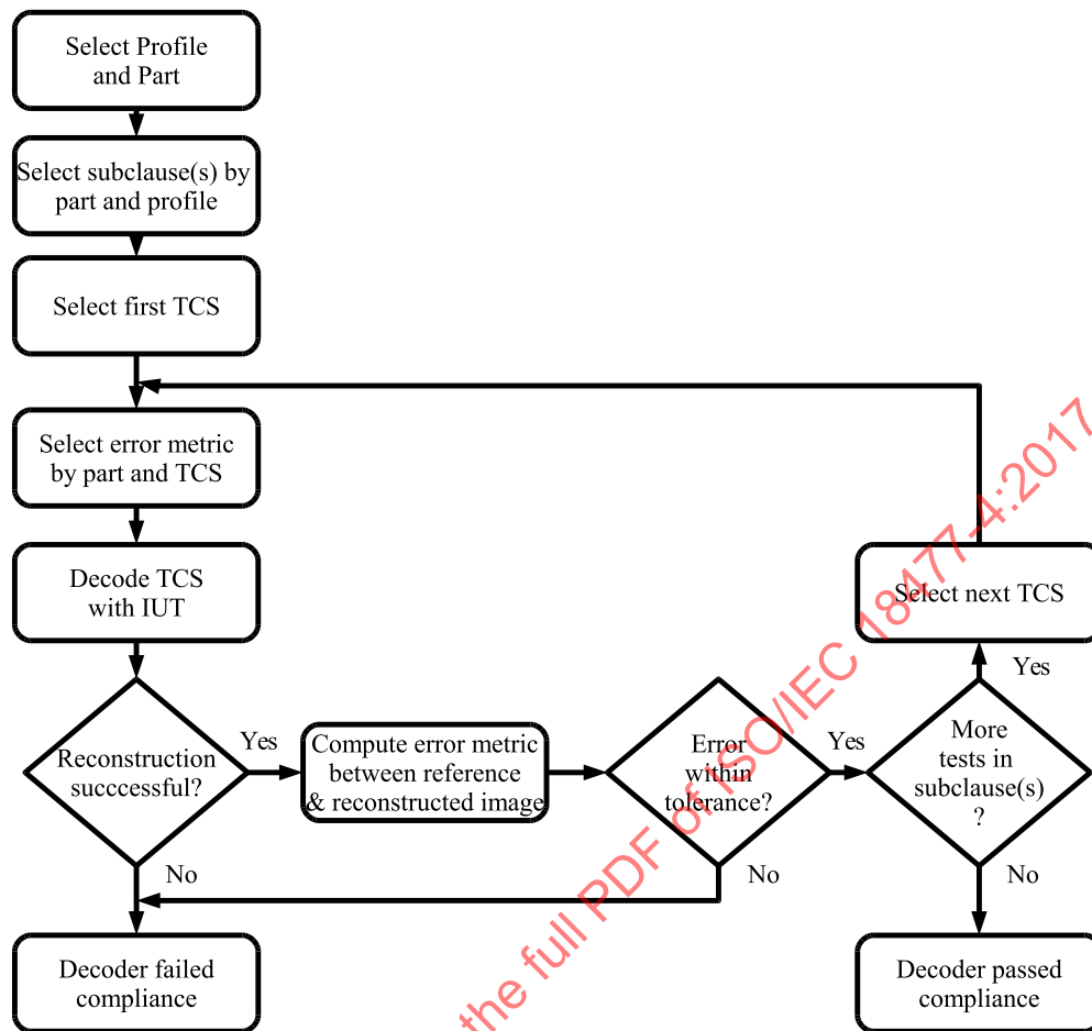
Figure A.1 — Decoder conformance test flow chart
