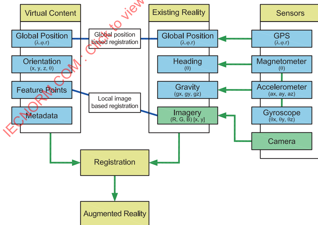
Figure A.8 — Overview of typical data flow in mobile outdoor AR
