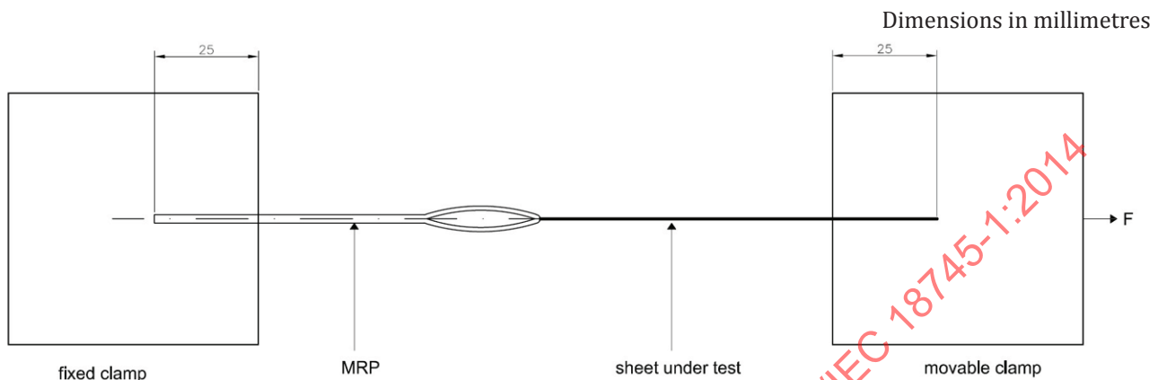
Figure 13 — Sheet Pull Apparatus
