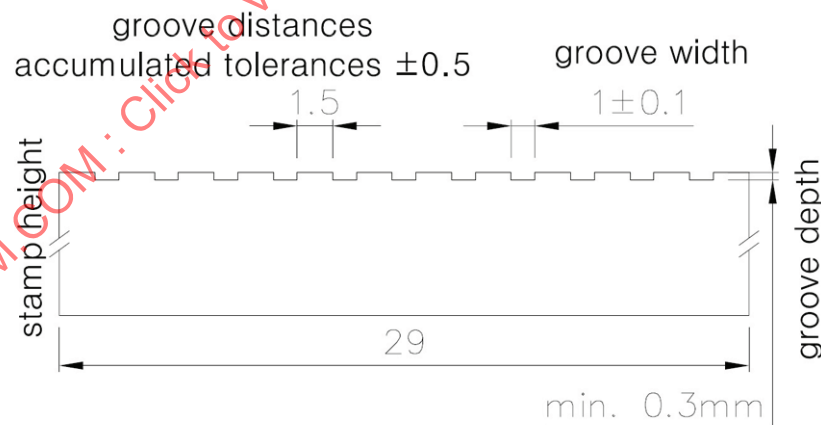
Figure 5 — Stamp geometry
