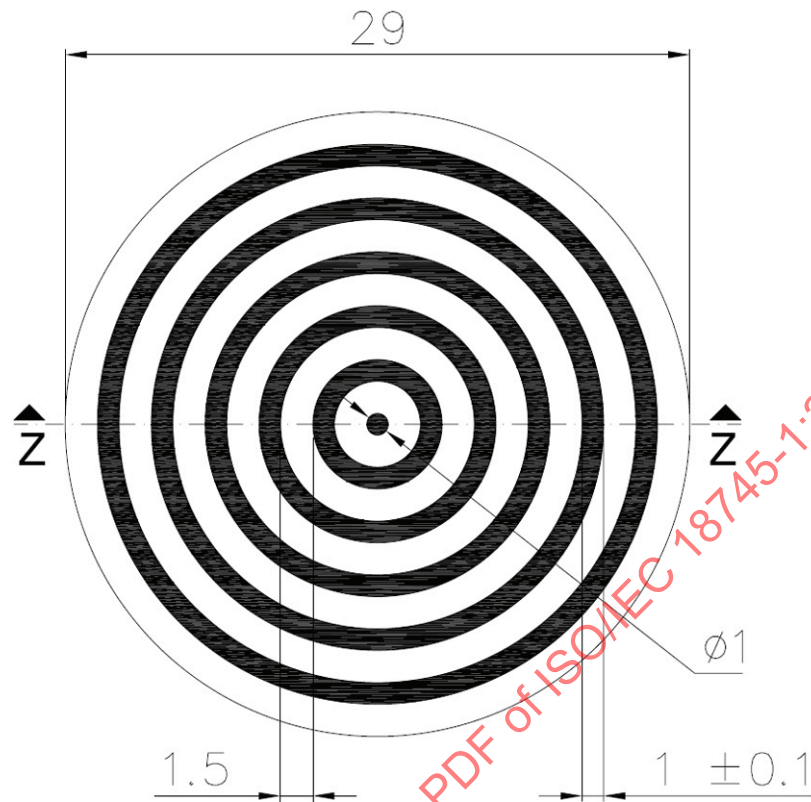
Figure 4 — Impact Pattern Resulting from Specified Stamp
