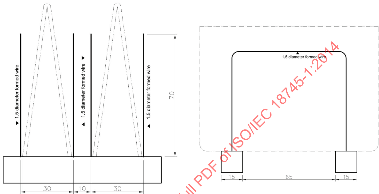
Figure 2 — MRP rack
