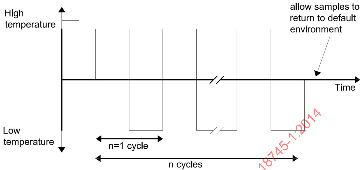
Figure 3 — Thermal Cycling
