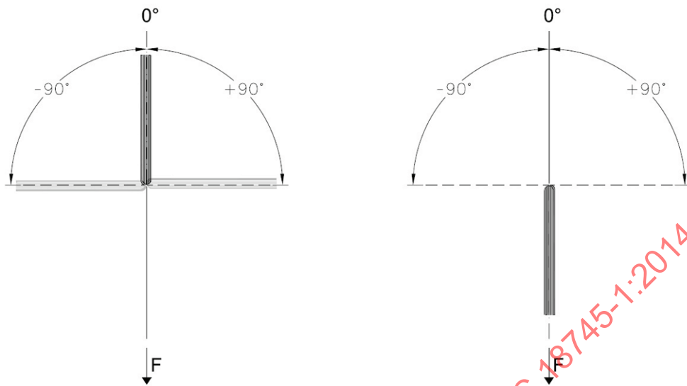
Figure 12 — Sheet Bending Illustration
