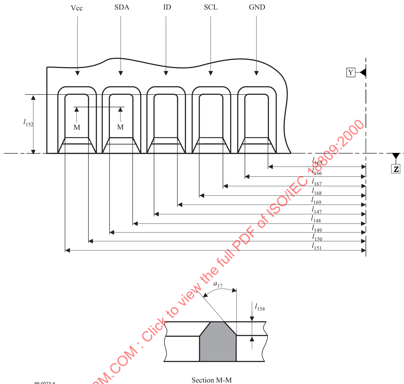
Figure 25 - MIC access holes, enlarged partial view, rear side
