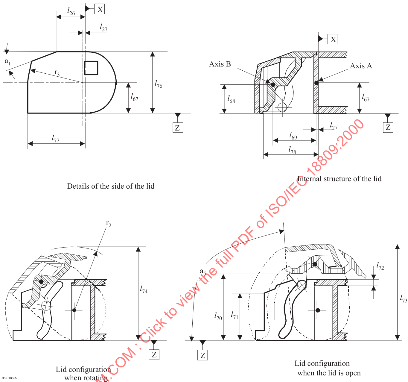
Figure 13 - Lid
