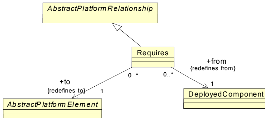
Figure 15.5 - ProvisioningRelations Class Diagram
