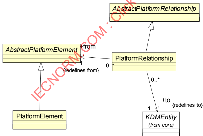
Figure 15.10 - ExtendedPlatformElements Class Diagram
