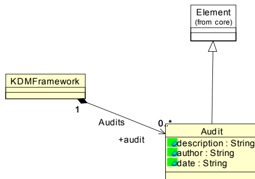
Figure 10.2 - Audit Class Diagram
