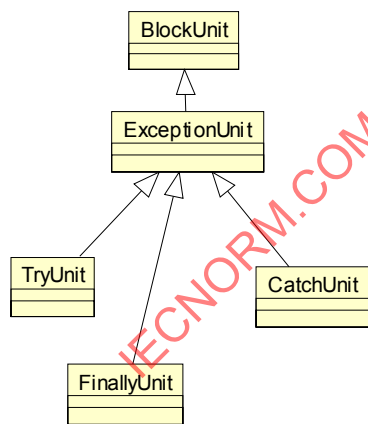
Figure 13.6 - ExceptionBlocks Class Diagram
