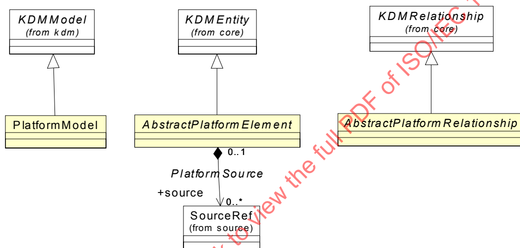
Figure 15.2 - PlatformInheritances Class Diagram
