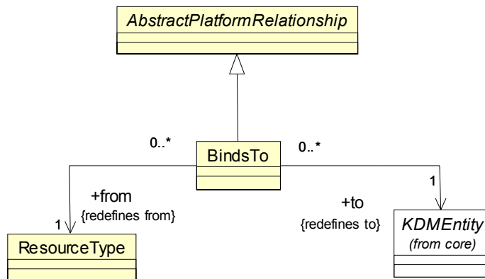
Figure 15.4 - PlatformRelations Class Diagram
