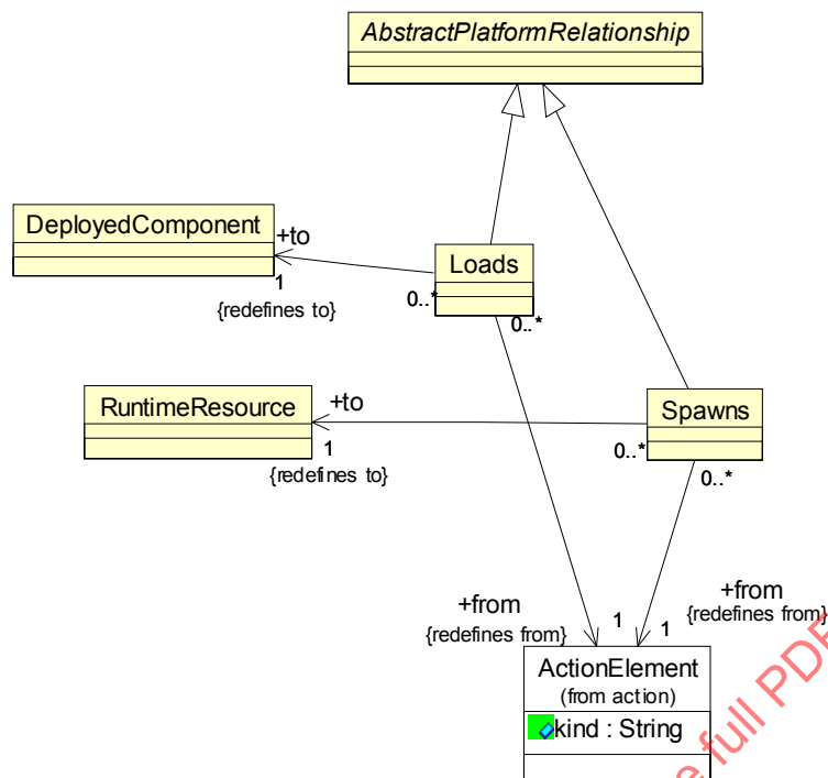
Figure 15.9 - RuntimeActions Class Diagram
