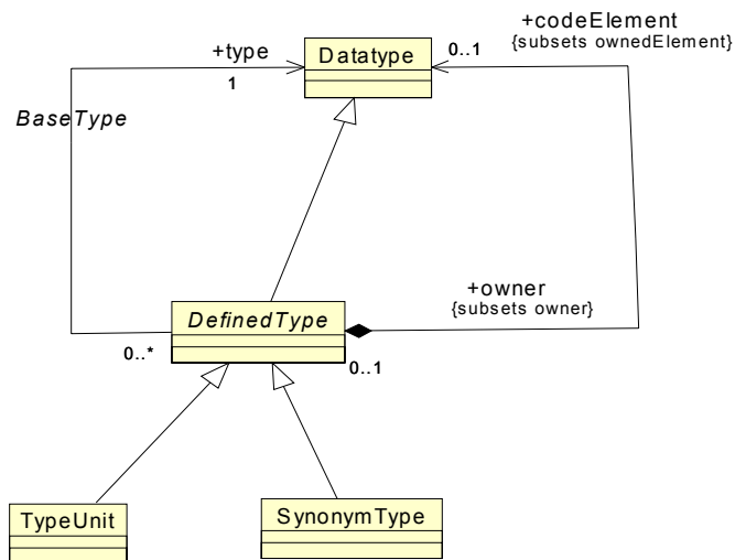
Figure 12.12 - DefinedTypes Class Diagram
