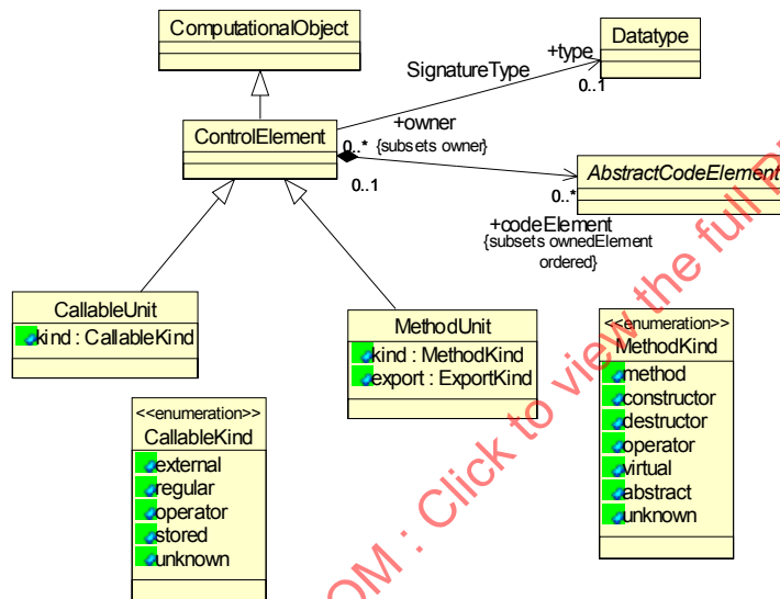
Figure 12.4 - ControlElements Class Diagram
