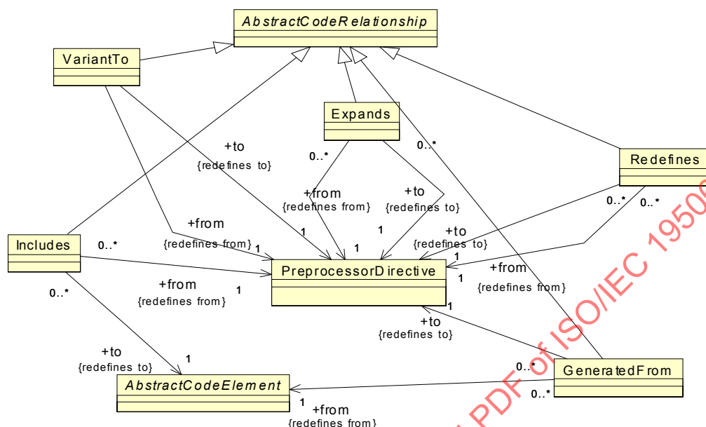
Figure 12.20 - PreprocessorRelations Class Diagram
