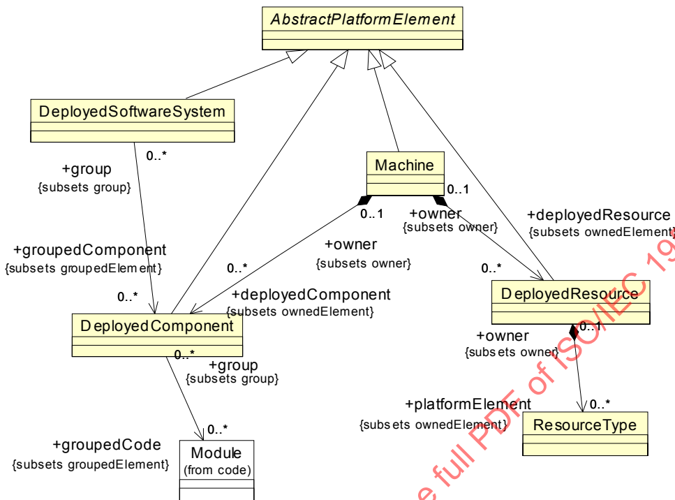
Figure 15.7 - Deployment Class Diagram
