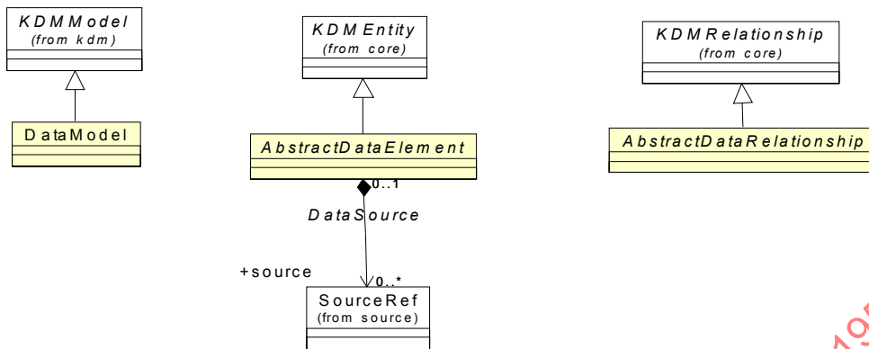
Figure 18.2 - DataInheritance Diagram
