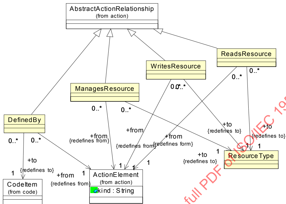
Figure 15.6 - PlatformActions Class Diagram
