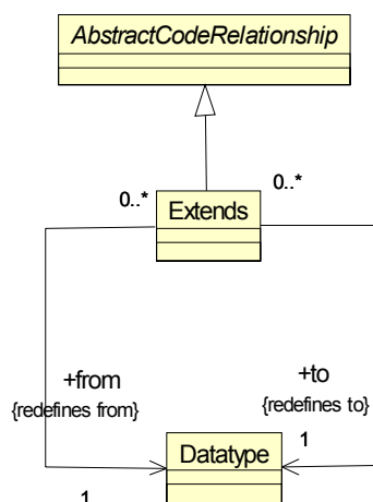
Figure 12.18 - ClassRelations Class Diagram
