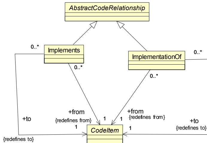
Figure 12.16 - InterfaceRelations Class Diagram
