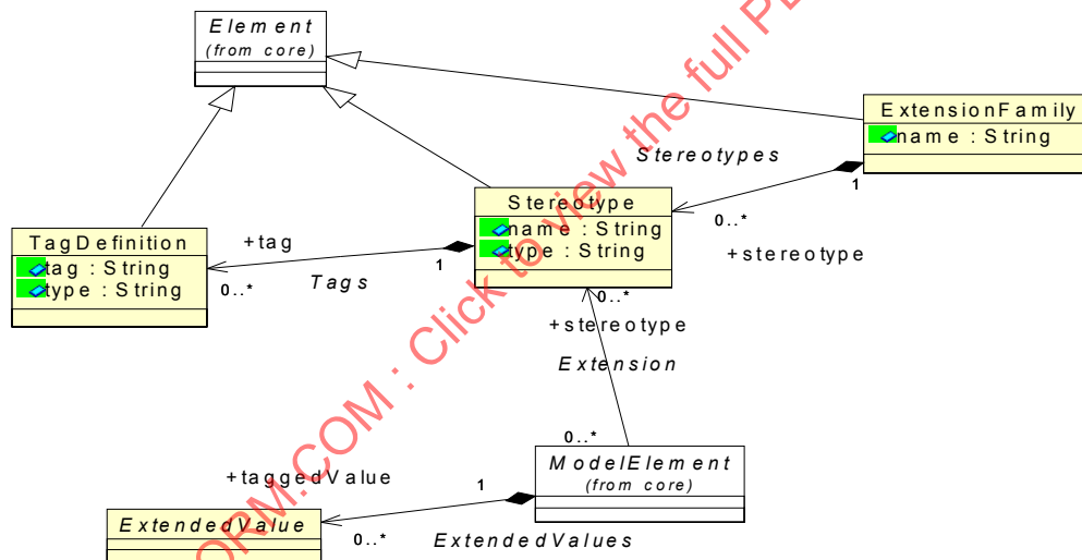
Figure 10.3 - Extensions Class Diagram
