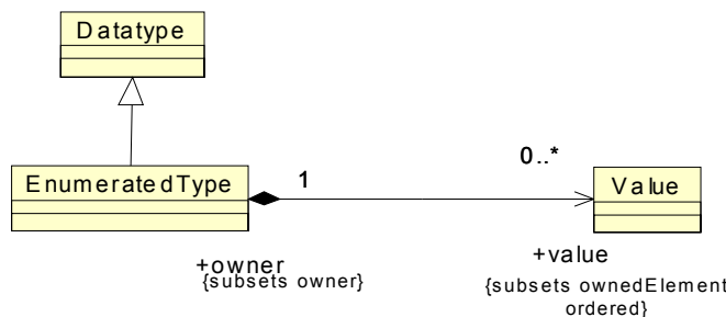
Figure 12.8 - EnumeratedTypes Class Diagram
