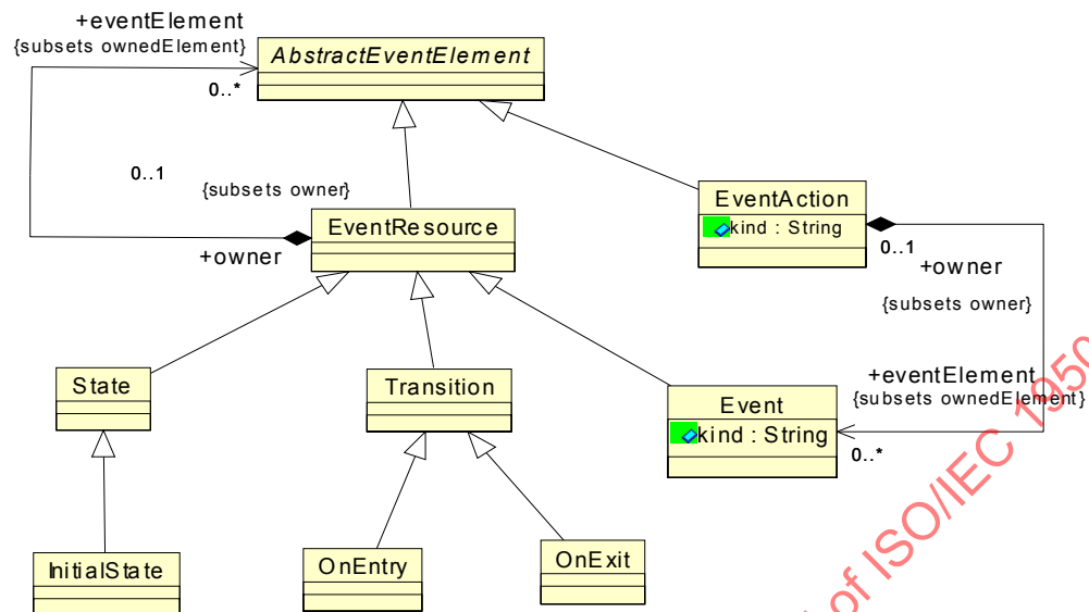
Figure 17.3 - EventResourcesClass Diagram
