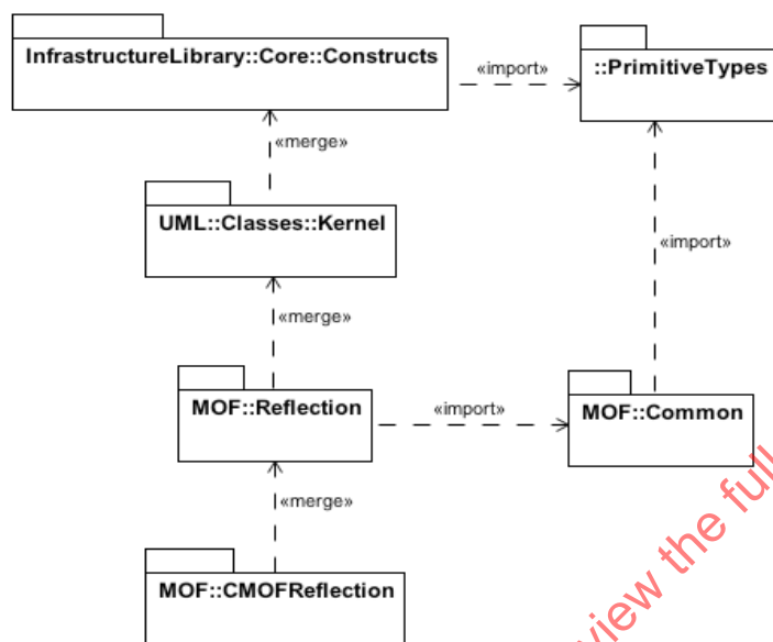
Figure 13.1 - CMOF Reflection
