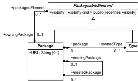
Figure 12.4 - EMOF Package
