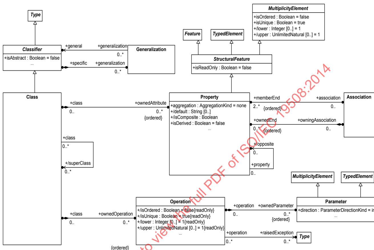
Figure 12.2 - EMOF Classes
