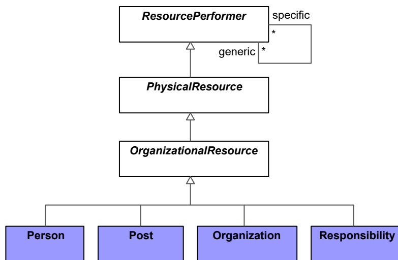
Figure 8:28 - Personnel Taxonomy
