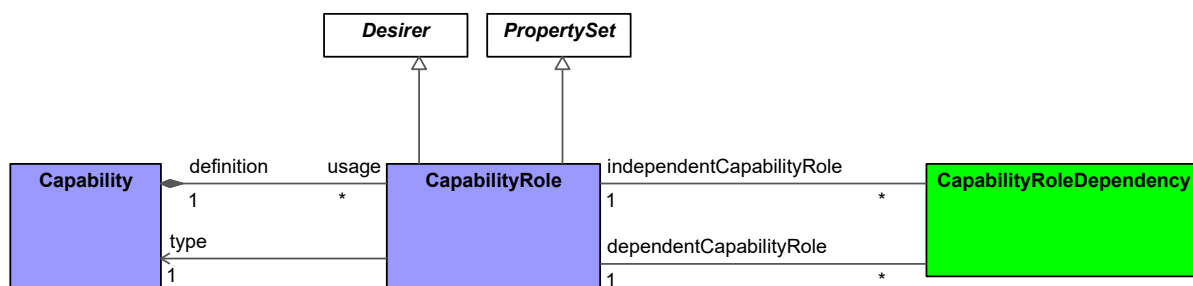
Figure 9:31 - CapabilityRole
