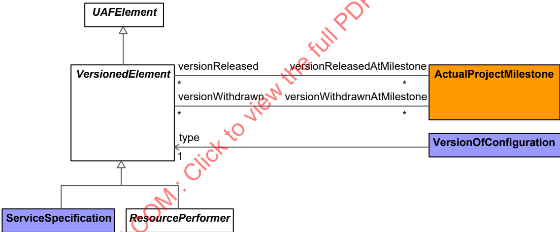
Figure 9:138 - VersionedElement
