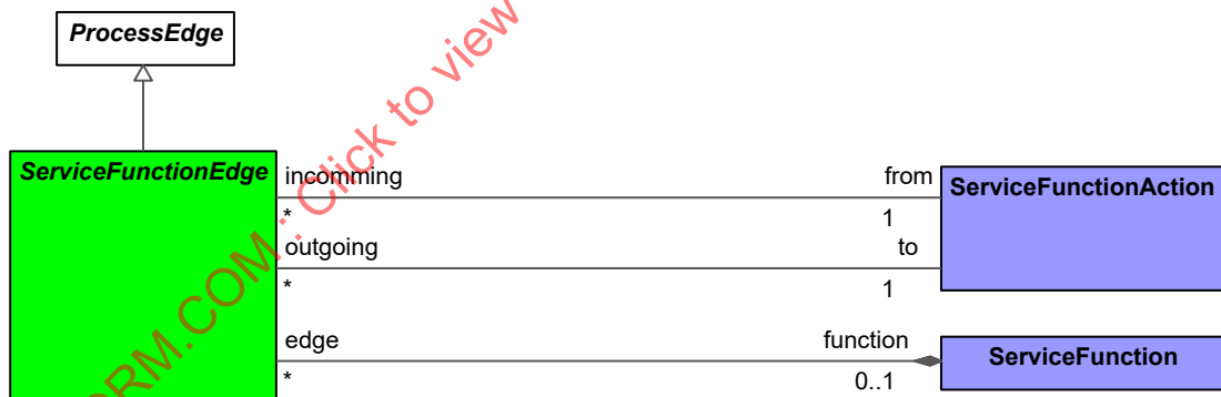
Figure 9:88 - ServiceFunctionEdge
