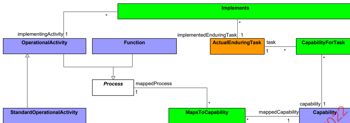
Figure 8:8 - Strategic Traceability
