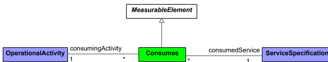
Figure 9:93 - Consumes
