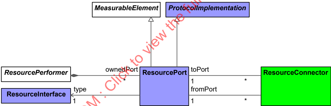
Figure 9:119 - ResourcePort
