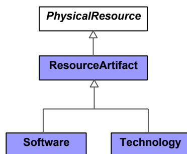
Figure 9:113 - ResourceArtifact
