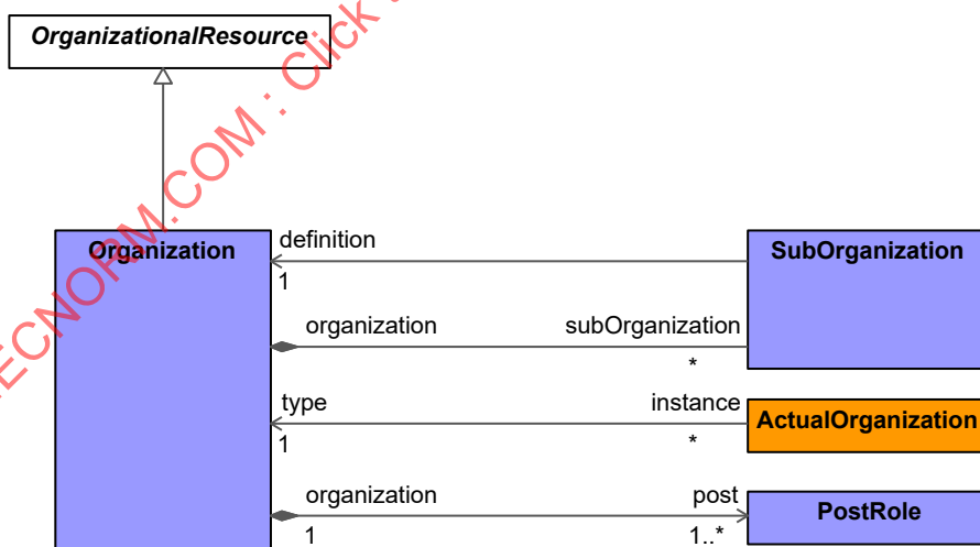
Figure 9:94 - Organization
