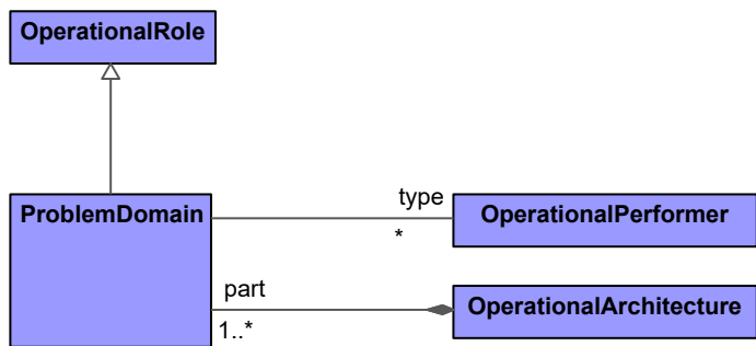
Figure 9:61 - ProblemDomain
