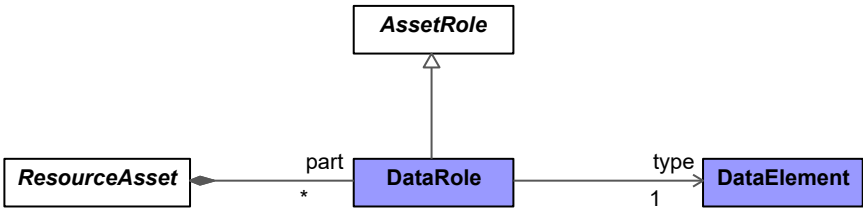
Figure 9:132 - DataRole
