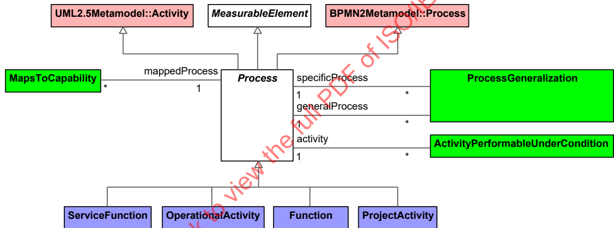
Figure 9:15 - Process
