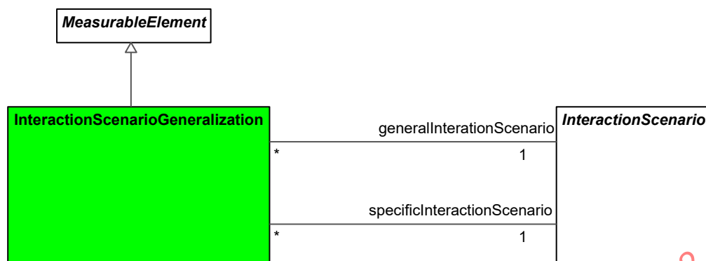
Figure 9:2 - InteractionScenarioGeneralization
