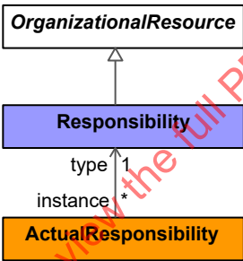
Figure 9:98 - Responsibility
