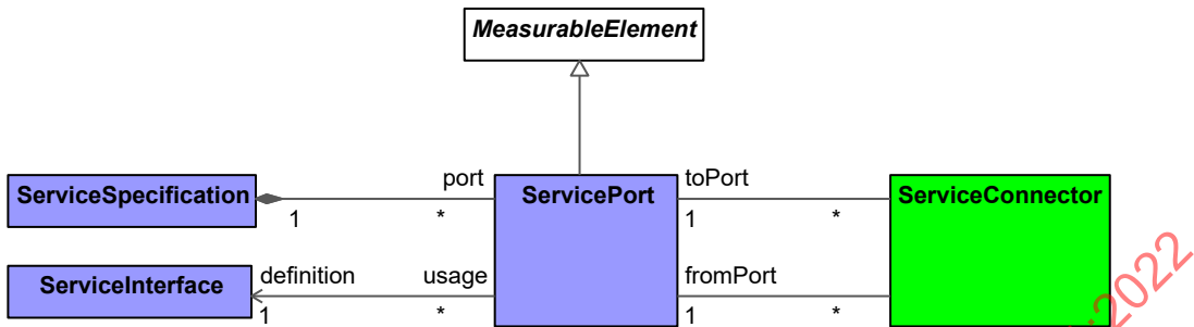
Figure 9:85 - ServicePort
