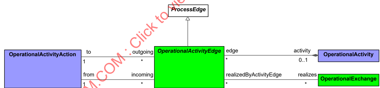
Figure 9:70 - OperationalActivityEdge
