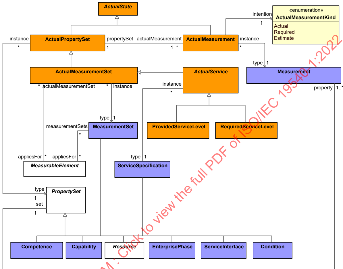
Figure 8:76 - Parameters: Measurements
