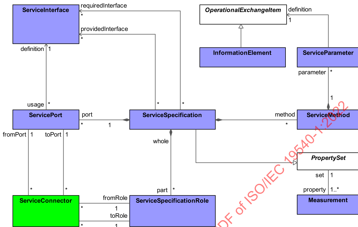
Figure 8:19 - Services Structure
