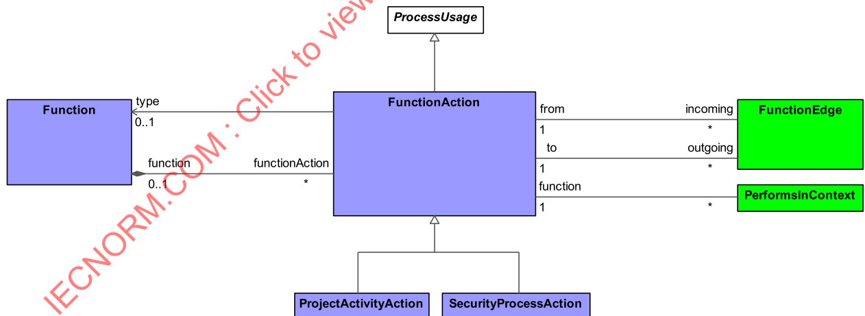
Figure 9:127 - FunctionAction
