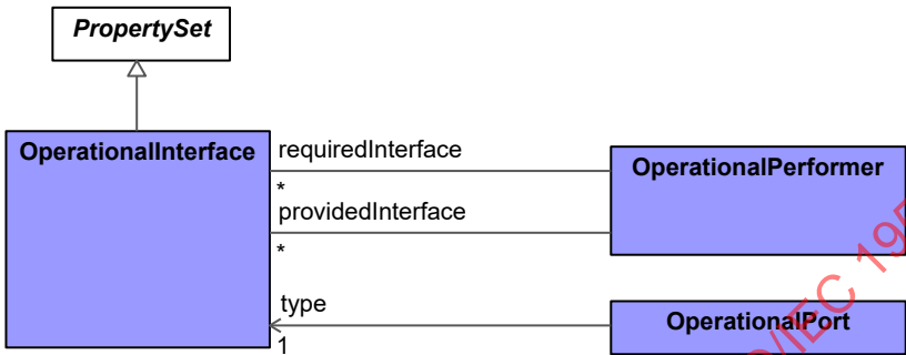
Figure 9:65 - OperationalInterface
