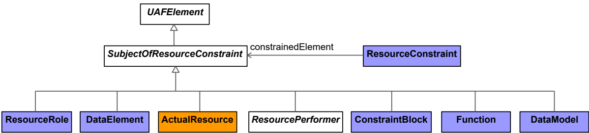
Figure 9:134 - SubjectOfResourceConstraint
