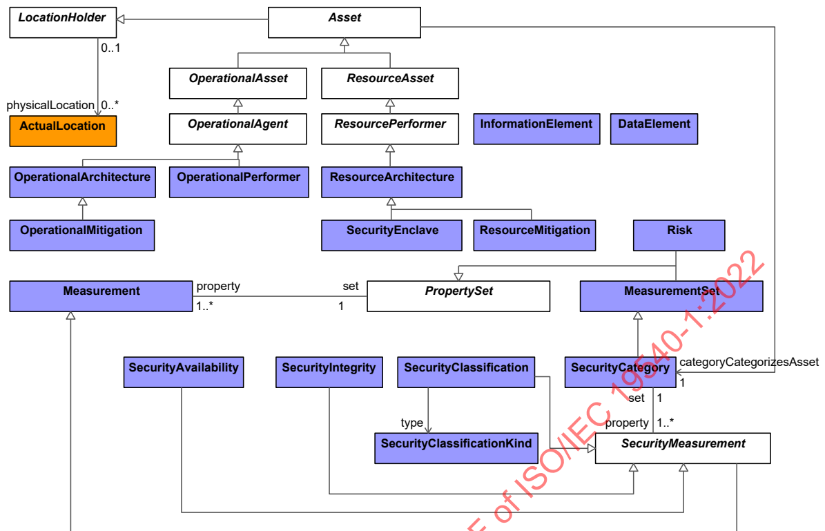
Figure 8:52 - Security Taxonomy
