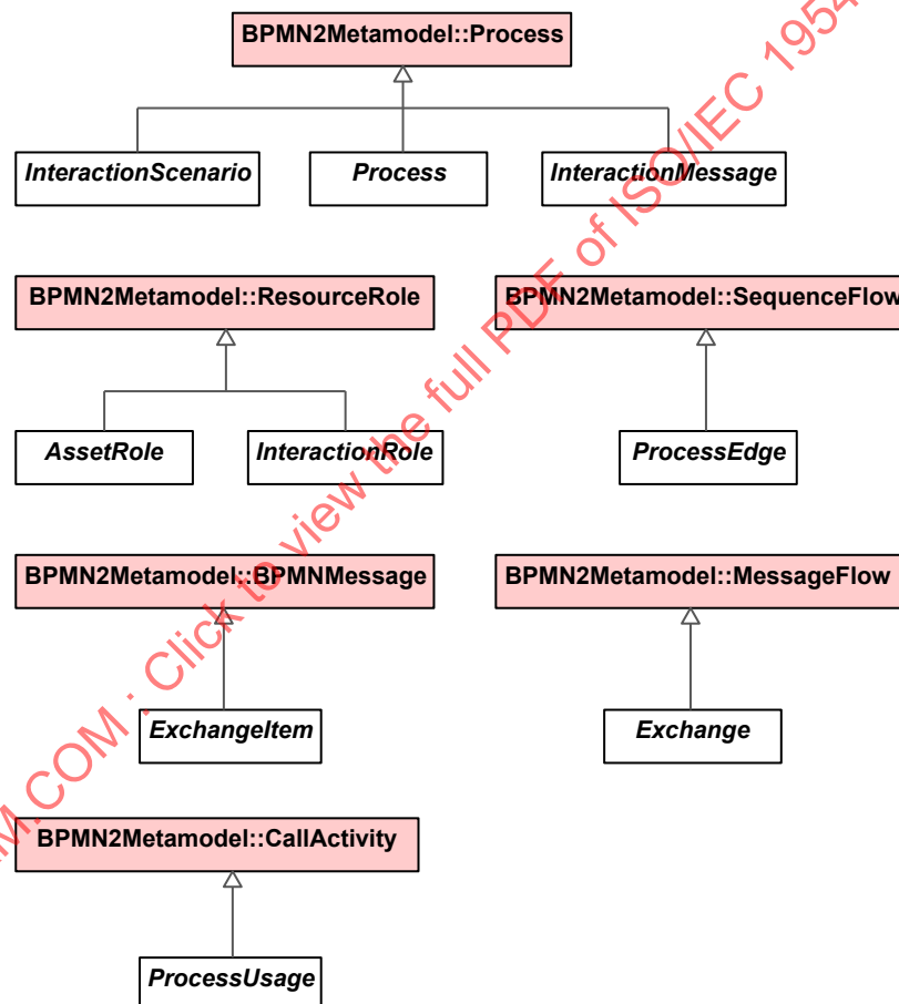
Figure 8:77 - BPMN
