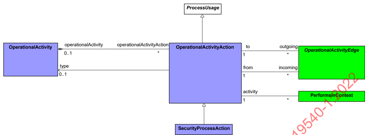
Figure 9:69 - OperationalActivityAction
