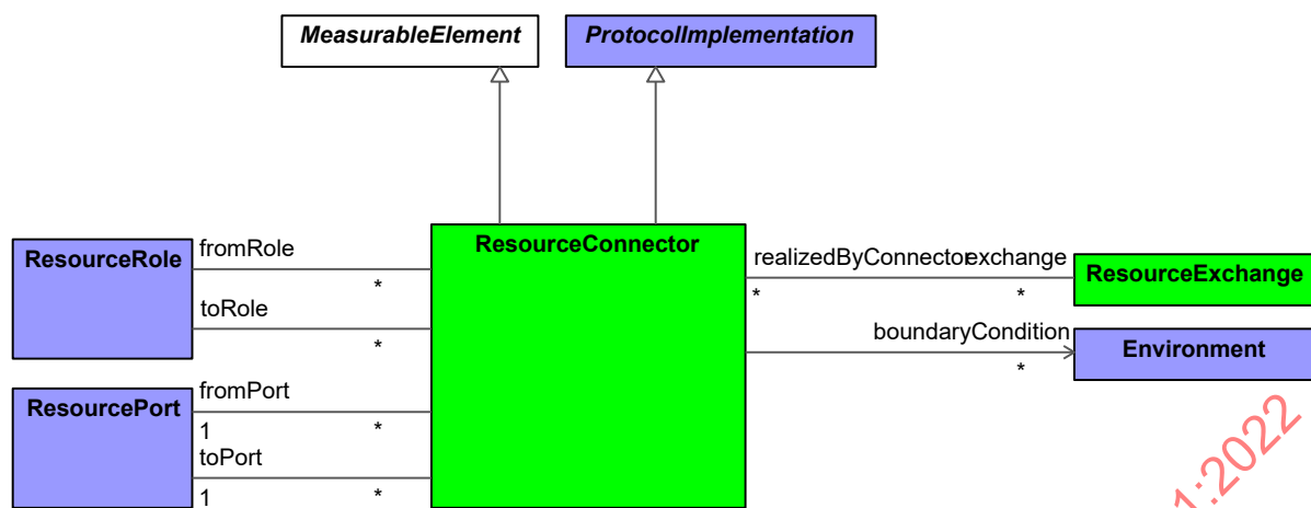
Figure 9:121 - ResourceConnector
