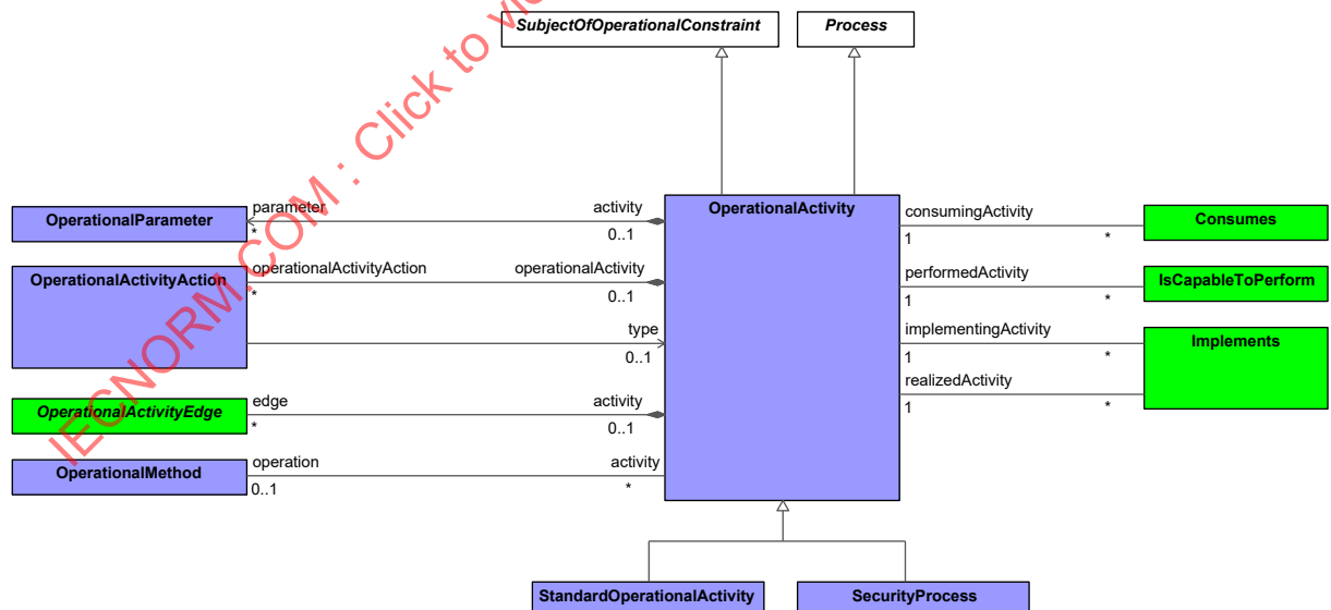
Figure 9:68 - OperationalActivity
