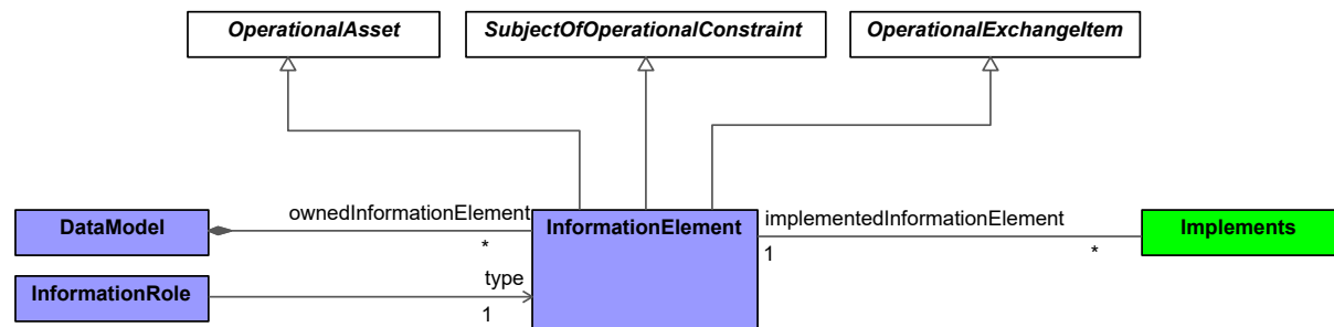
Figure 9:75 - InformationElement
