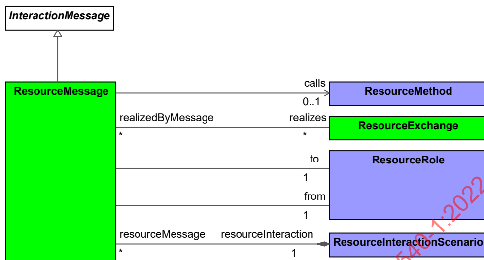
Figure 9:130 - ResourceMessage
