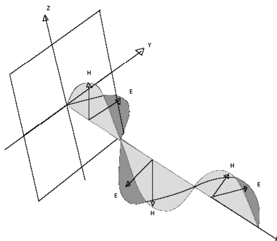
Figure 2 — Electromagnetic field
