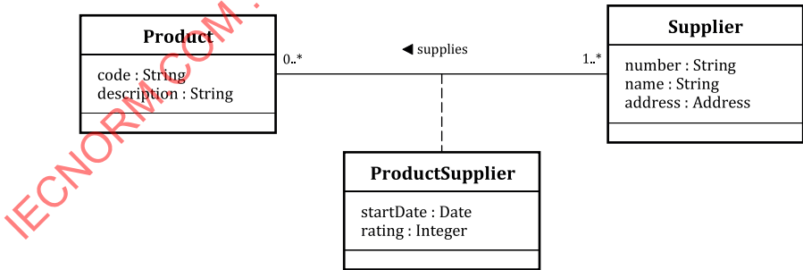
Figure A.1 — Example UML Class Diagram for the Product Supplier concept
