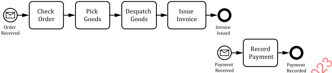
Figure A.5 — Example workflow model for the Handle Order process
