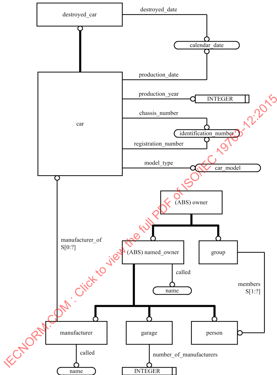
Figure D.1 — Example information model drawn in EXPRESS-G
