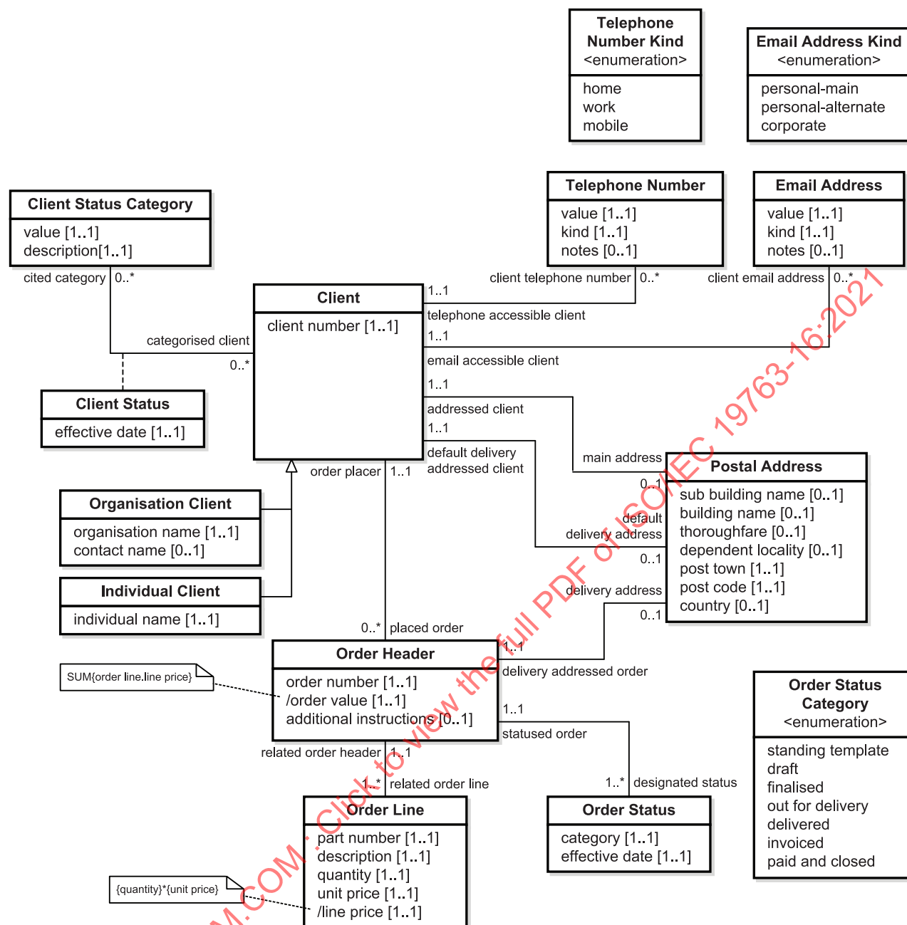
Figure C.6 — UML class diagram for the order processing scenario
