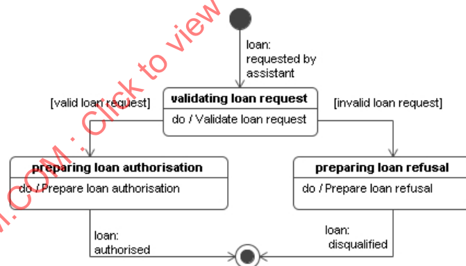
Figure A.12 – State diagram for Library system role in the interaction Process loan
