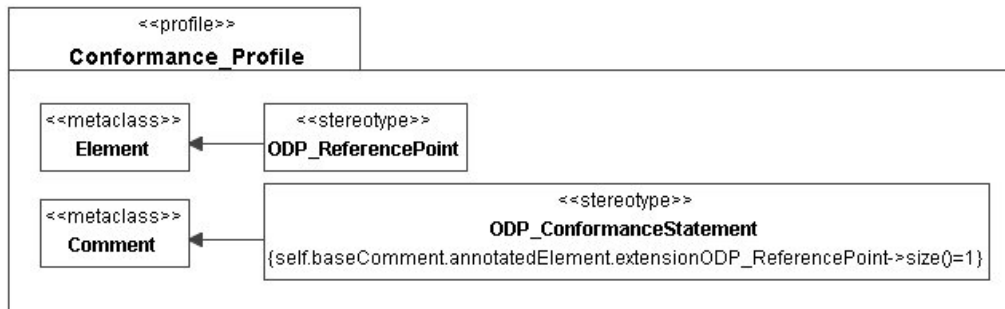
Figure 39 – UML profile for conformance
