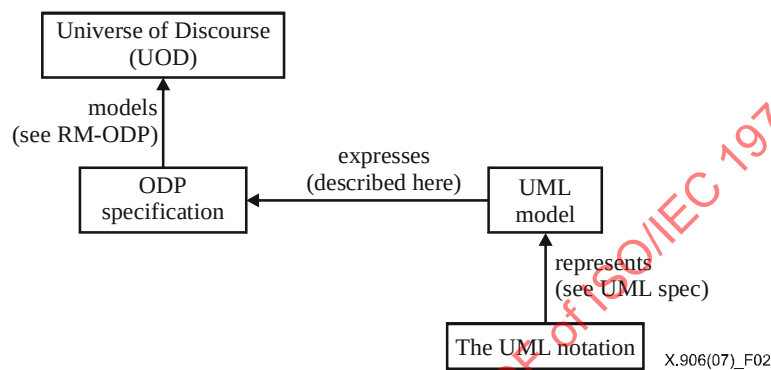
Figure 2 – Relationships between UOD, ODP specifications and UML models
