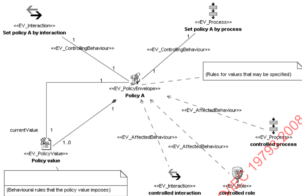
Figure 9 – Pattern for UML expression of a policy
