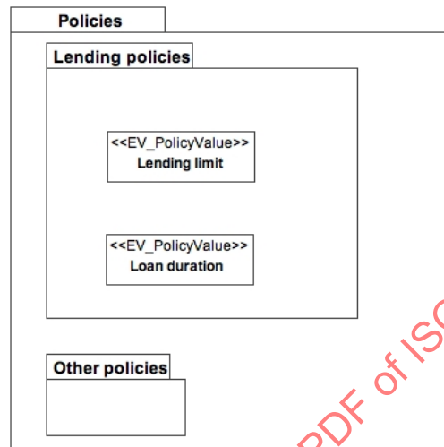
Figure A.18 – Structure of the Policies package
