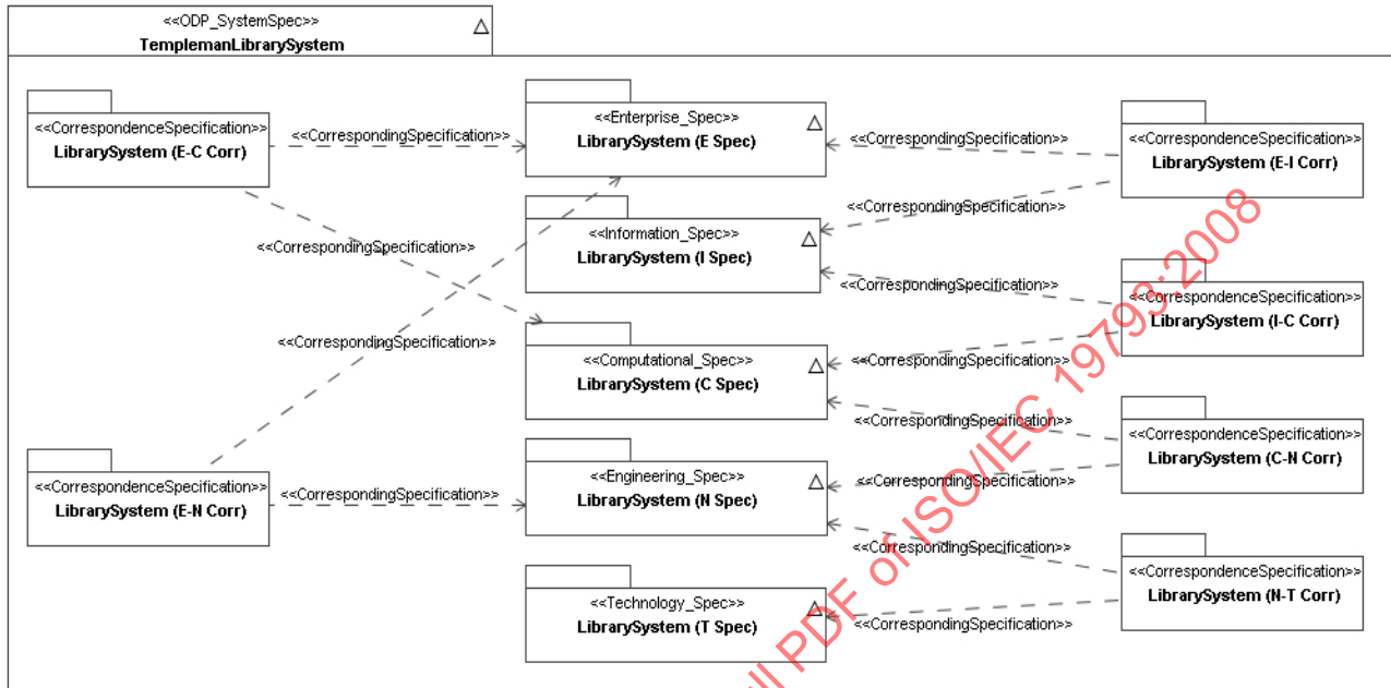
Figure A.1 – UML specification of the ODP system
