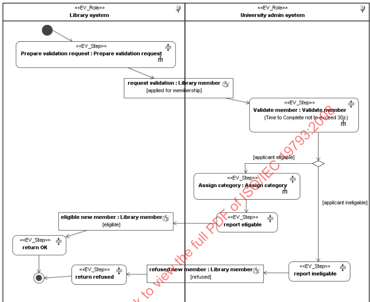
Figure A.8 – Validate member sub-process
