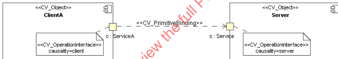
Figure 21 – An explicit primitive binding between two interfaces
