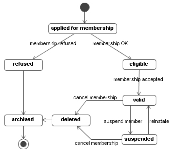
Figure A.17 – States of the Library member enterprise object
