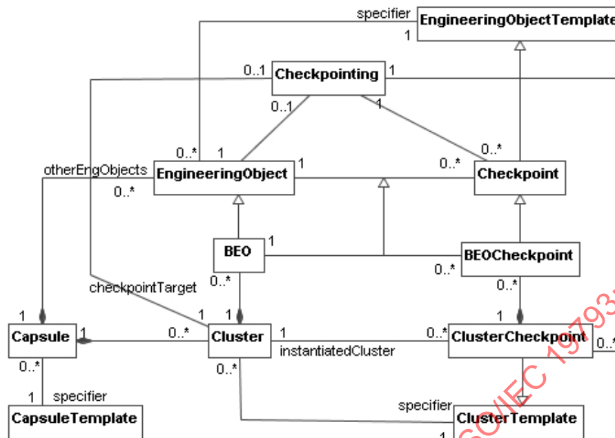
Figure 31 – Engineering language model – Checkpoints
