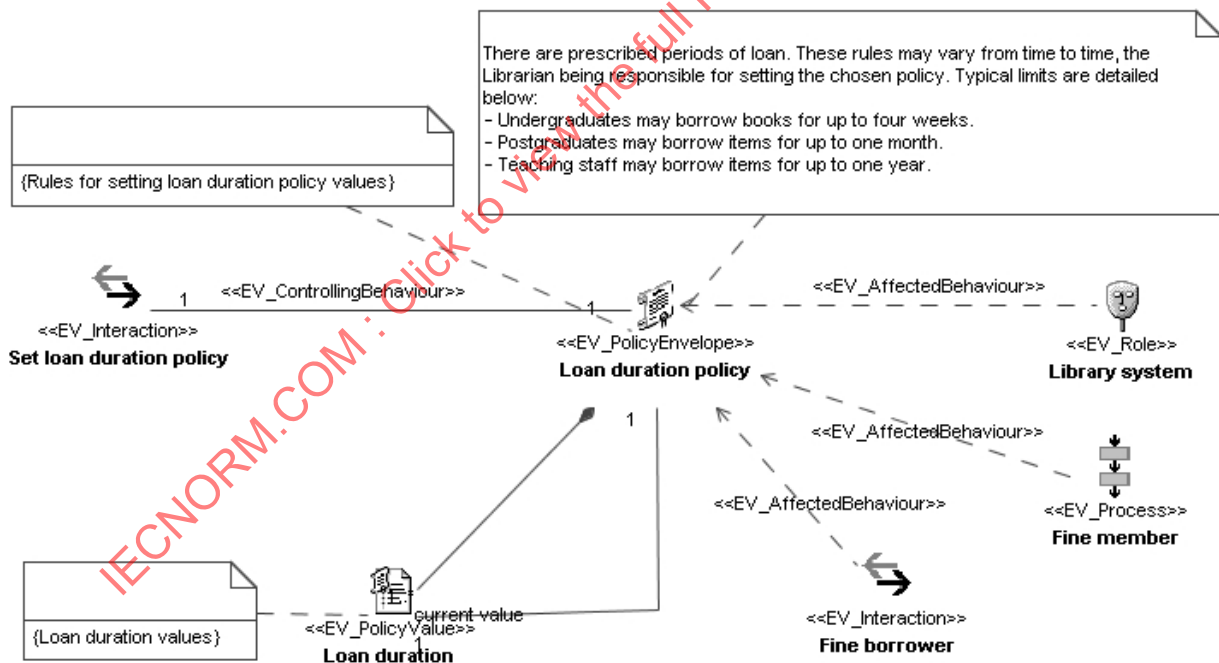
Figure A.20 – Examples of policy expressions: Loan duration policy
