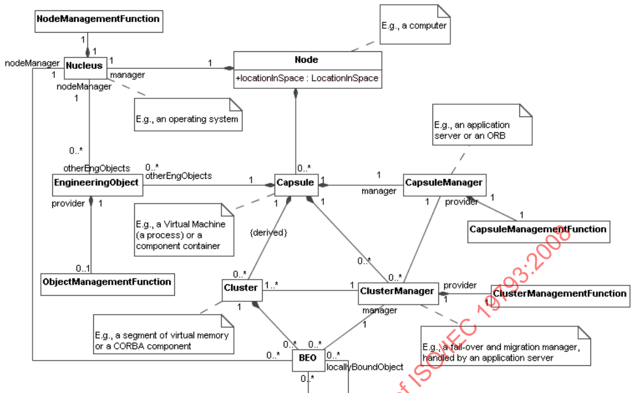
Figure 27 – Engineering language – Basic concepts
