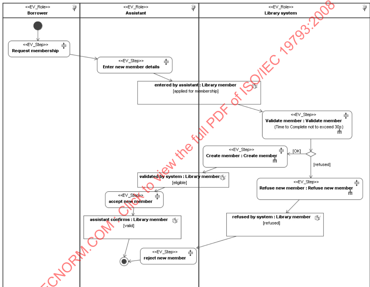
Figure A.7 – Add member process
