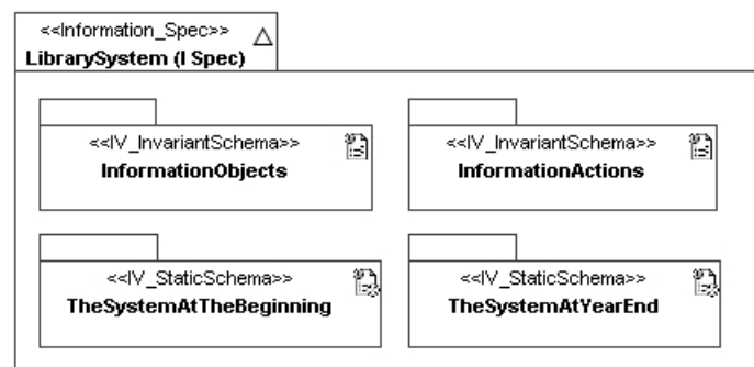
Figure A.23 – Structure of the information viewpoint specification of the Library system (excerpt)
