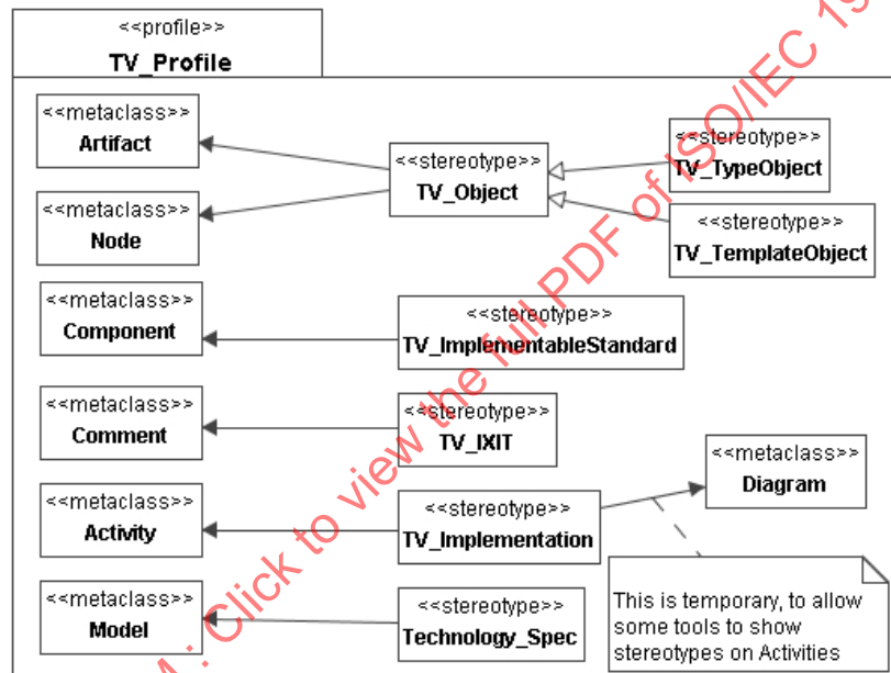
Figure 36 – Graphical representation of the technology language profile (using the UML notation)
