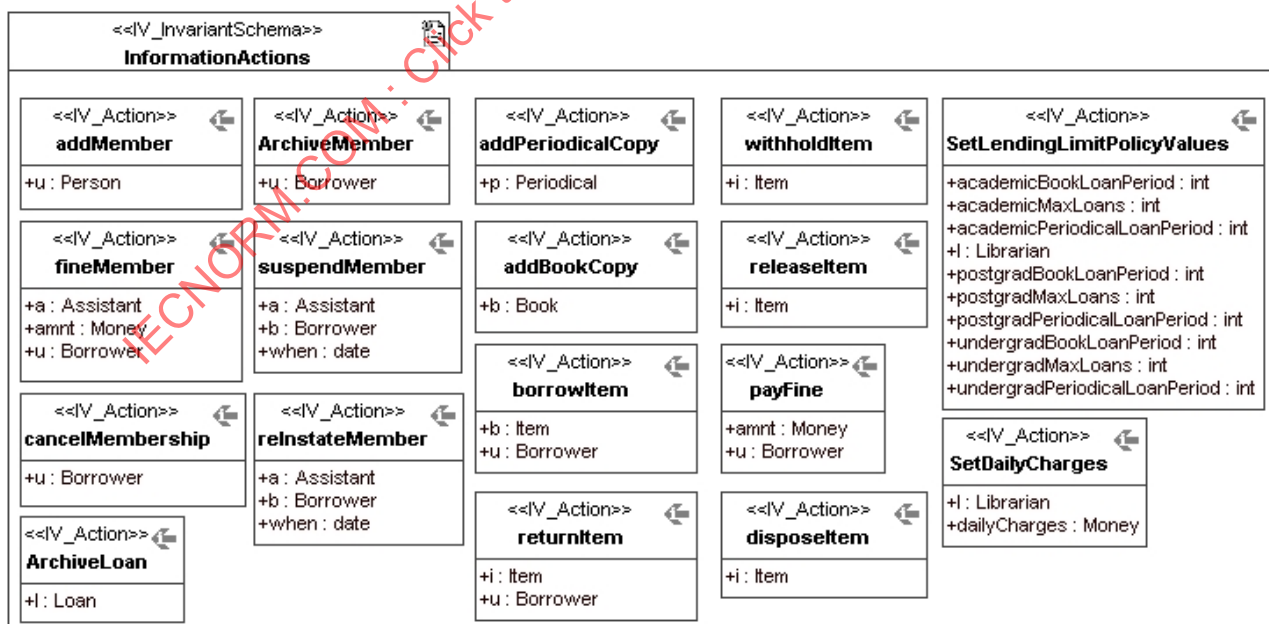
Figure A.25 – Action types of the information viewpoint specification of the Library system
