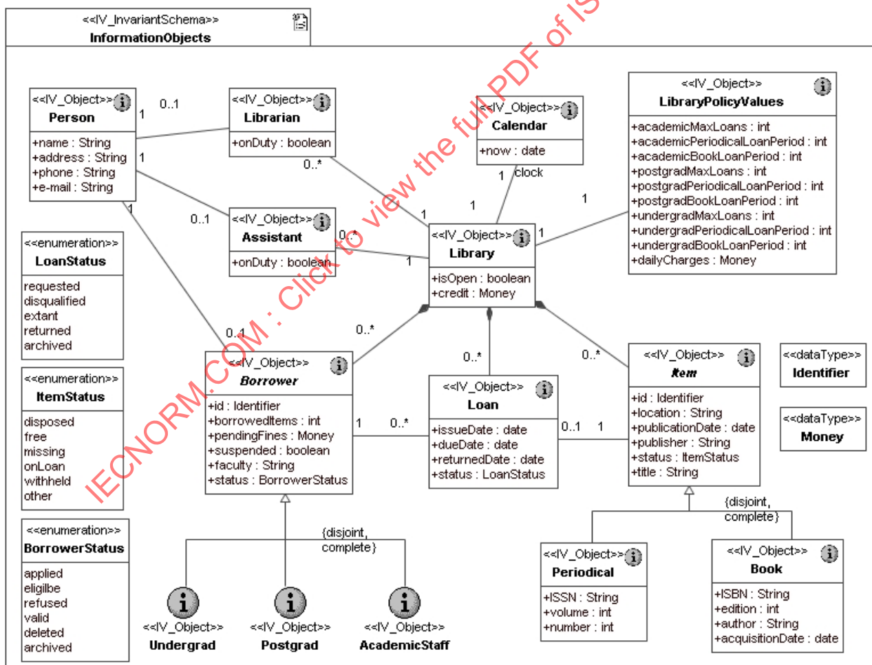
Figure A.24 – Object types of the information viewpoint specification of the Library system
