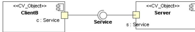
Figure 23 – An implicit primitive binding between two interfaces
