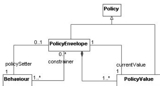
Figure 6 – Additional policy concepts
