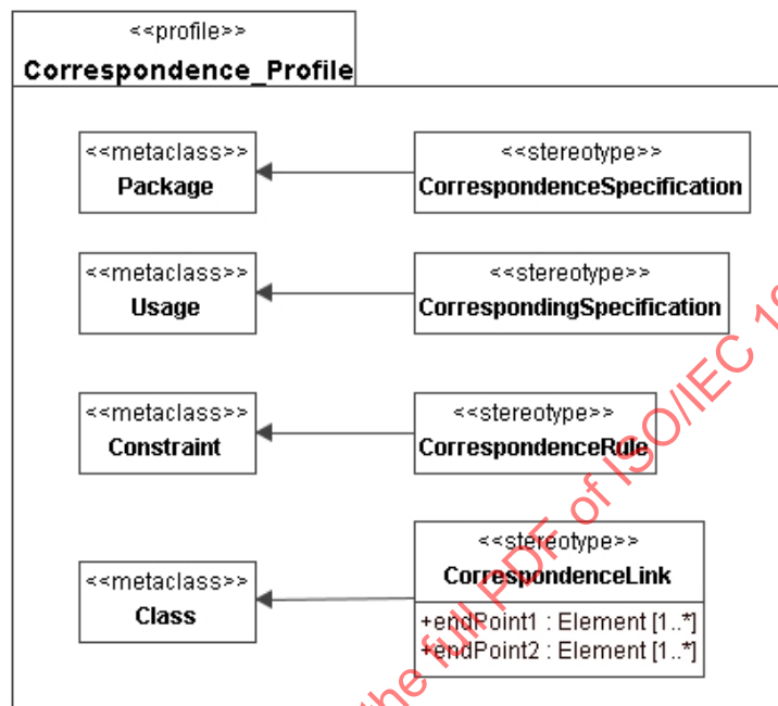
Figure 38 – Graphical representation of the UML profile for correspondences specifications
