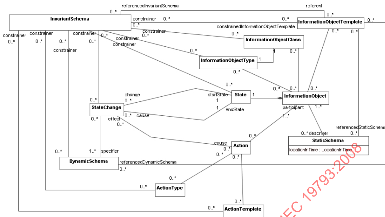
Figure 15 – Information language concepts
