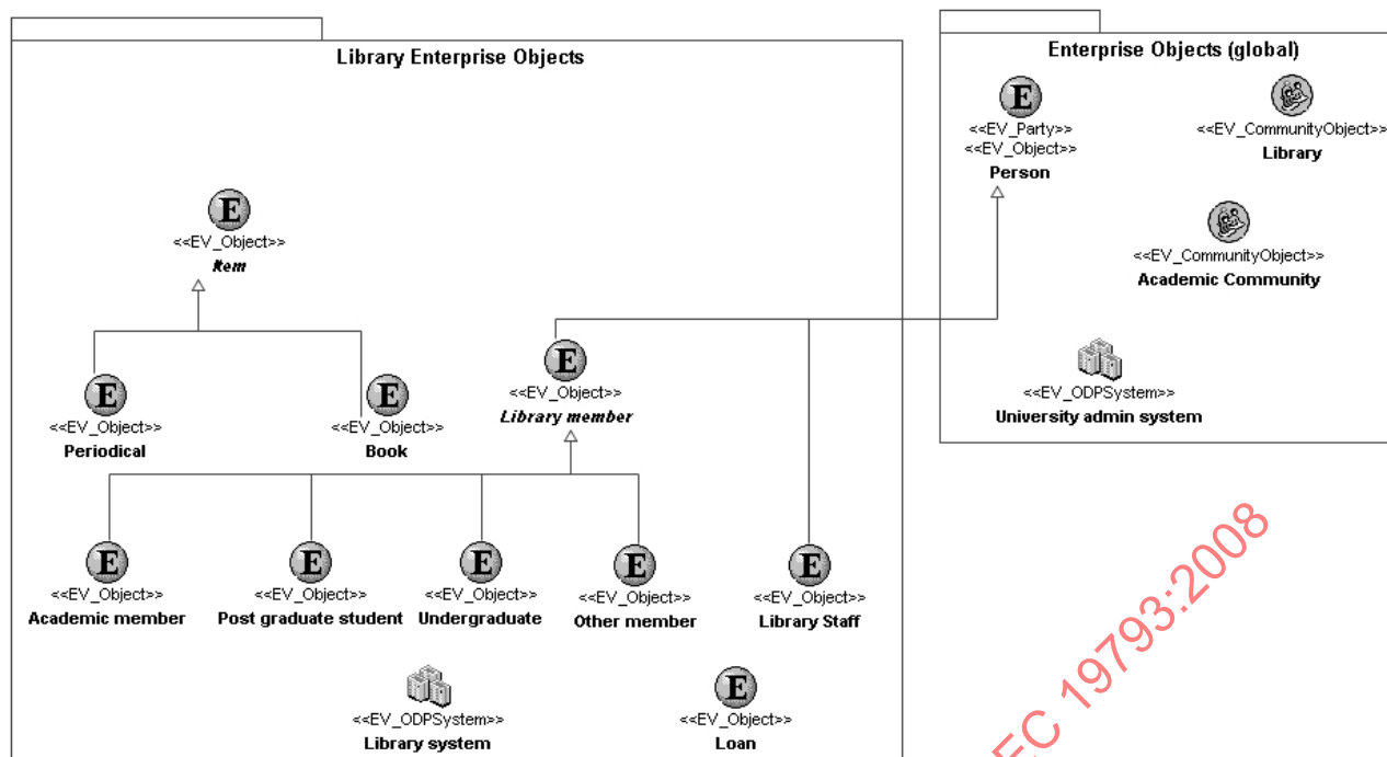
Figure A.15 – Enterprise objects
