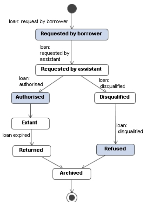
Figure A.16 – States of the Loan enterprise object
