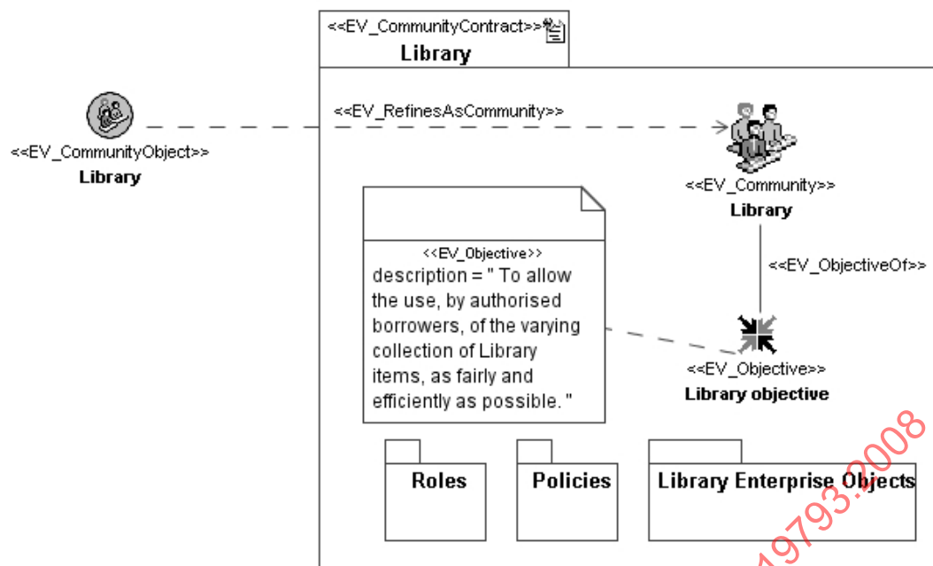
Figure A.4 – UML specification of the Library community
