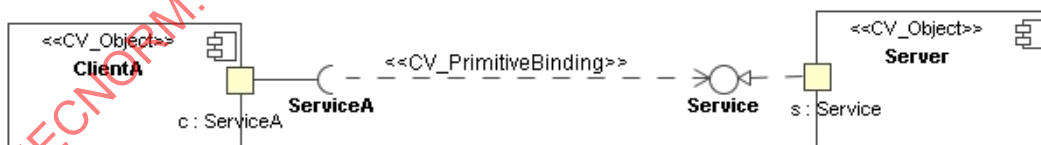
Figure 22 – An explicit primitive binding between two interfaces showing their interface signatures
