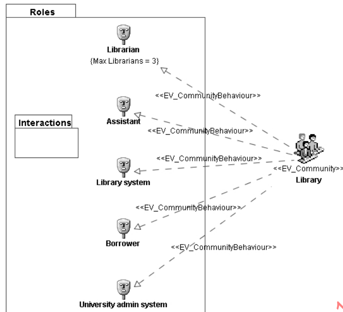
Figure A.9 – Library community roles
