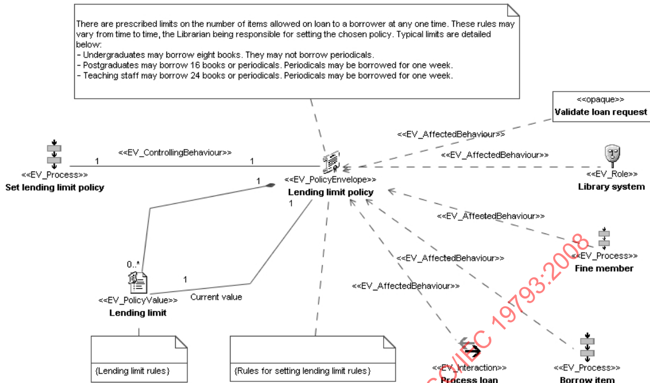
Figure A.19 – Examples of policy expressions: Lending limit policy
