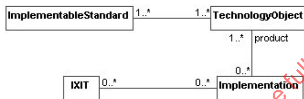
Figure 35 – Model of the technology language
