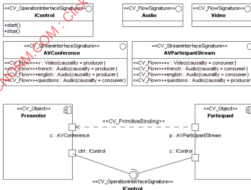
Figure 24 – An example of the specification of flows
