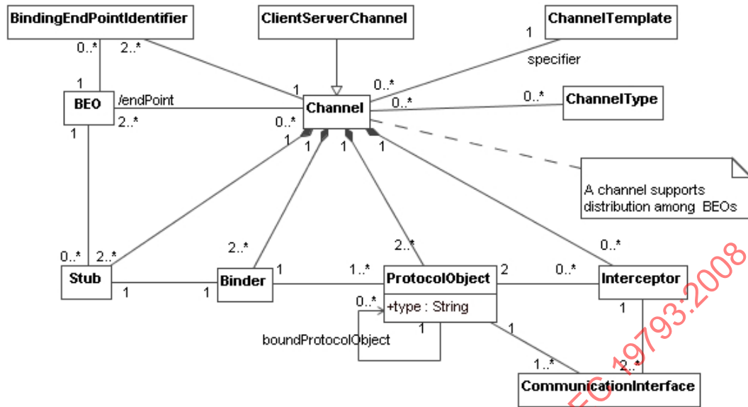
Figure 28 – Engineering language model – Channels
