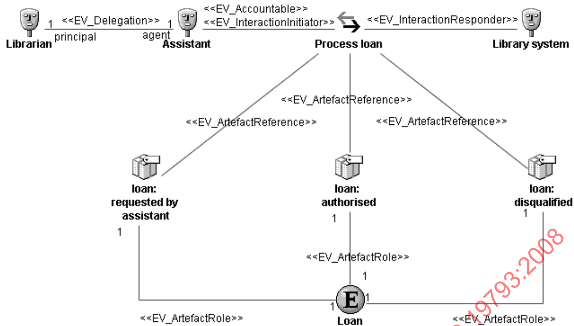
Figure A.11 – Process Loan interaction
