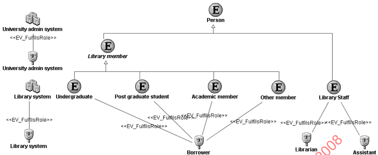
Figure A.13 – Actor Role fulfilment and assignment rules
