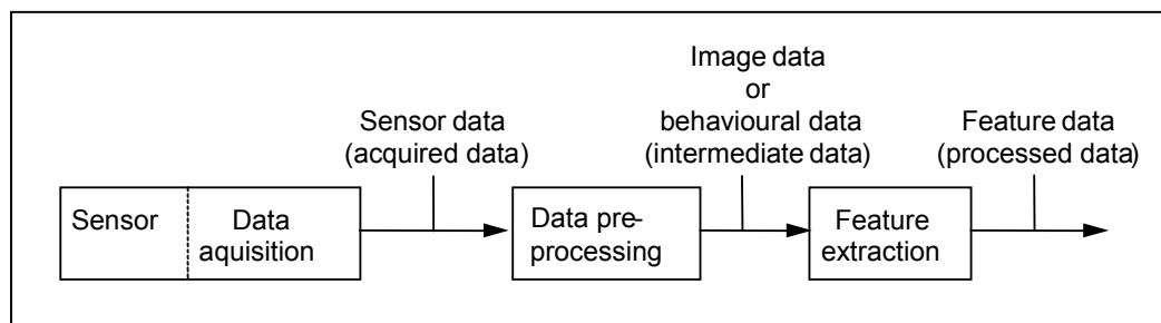
Figure 4 – Sensor data, image/behavioural data and feature data
