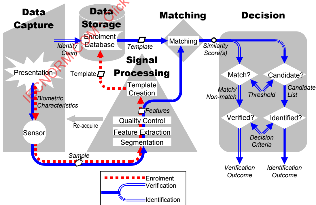
Figure 2 — Components of general biometric system
