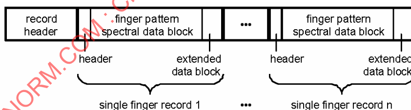
Figure 5 — Finger pattern spectral data record
