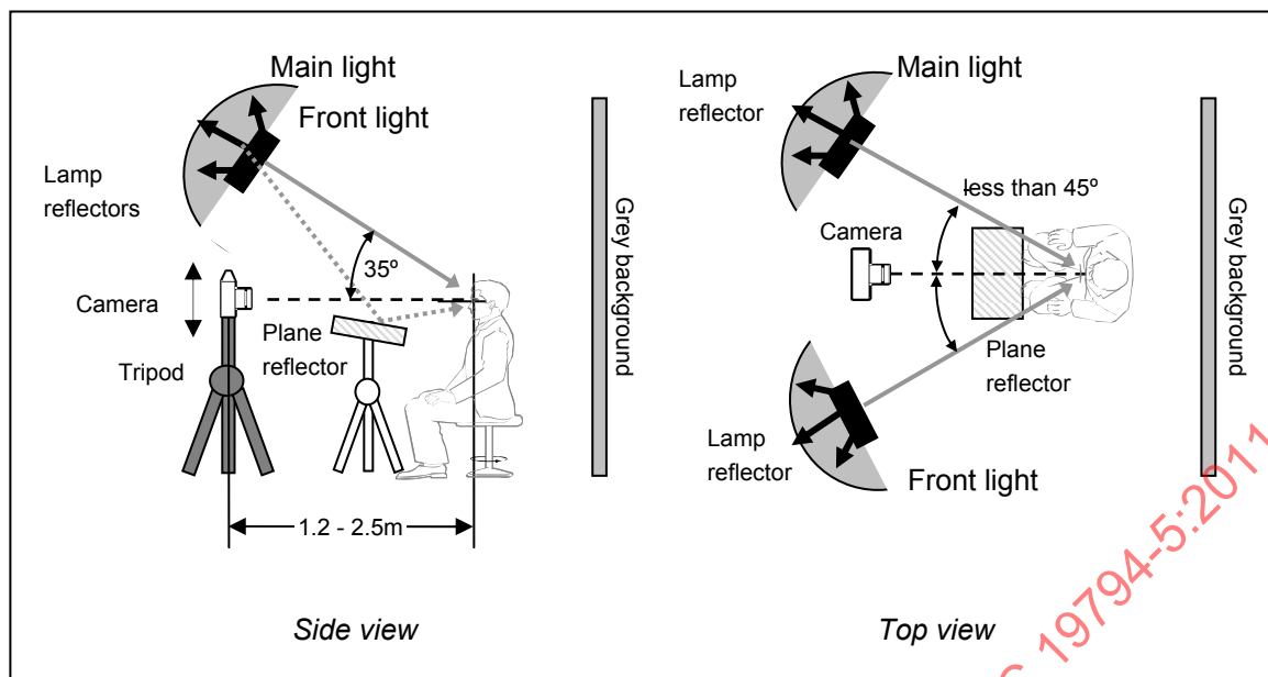
Figure C.5 — Lighting arrangement for a photo studio with dual front lights
