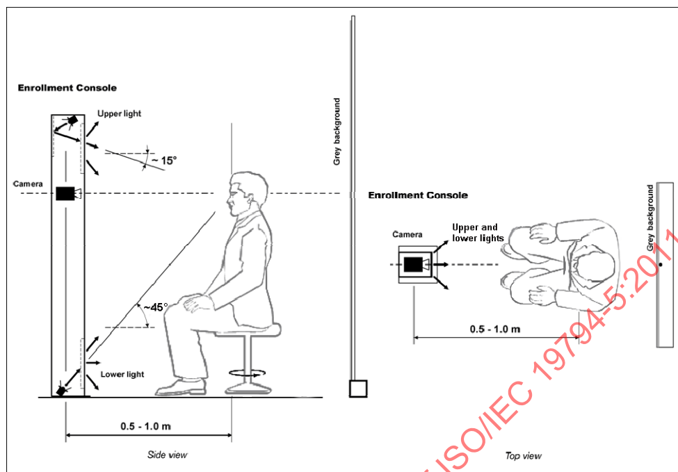
Figure C.10 — Recommended placements of subject, camera, and lights in a registration office environment
