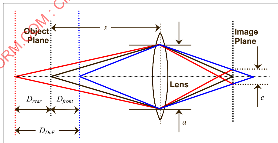
Figure C.1 — Dimensions for depth-of-field calculations
