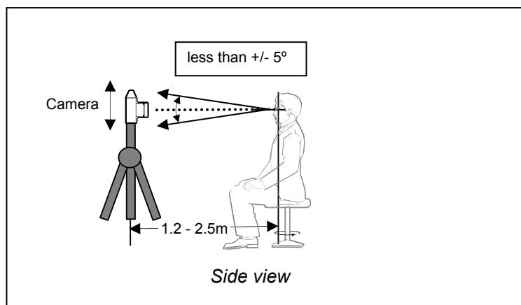
Figure C.2 — Preferred distance and alignment of camera and subject
