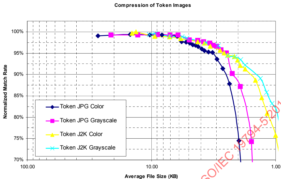
Figure B.9 — Identix, compression Token images versus face recognition performance
