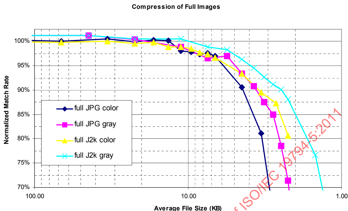
Figure B.6 — ZN Vision Technologies, compression of Full Frontal Images versus face recognition performance
