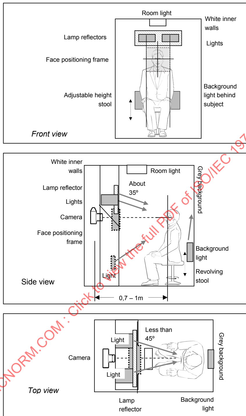
Figure C.7 — Recommended placements of subject, camera, and lights in a photo booth
