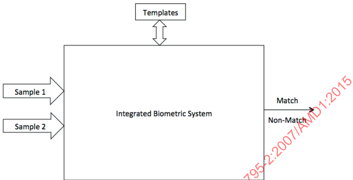
Figure F.2 — Fusion in an integrated multimodal system with decision output
