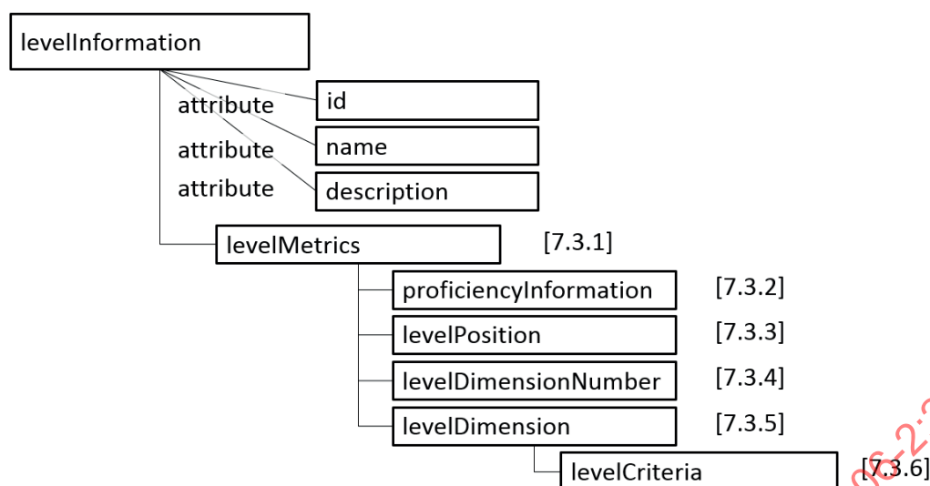
Figure 5 — Level information model
