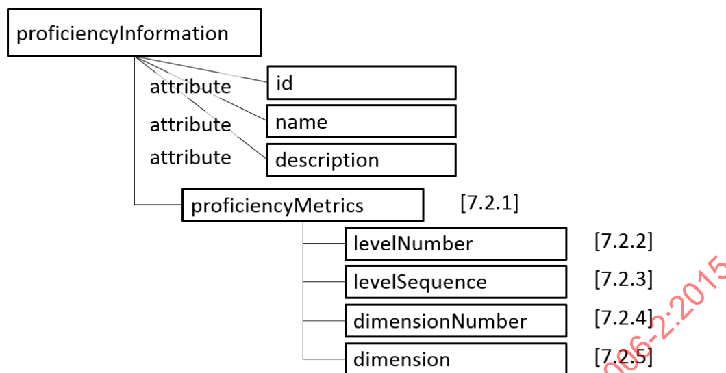
Figure 4 — Proficiency information model
