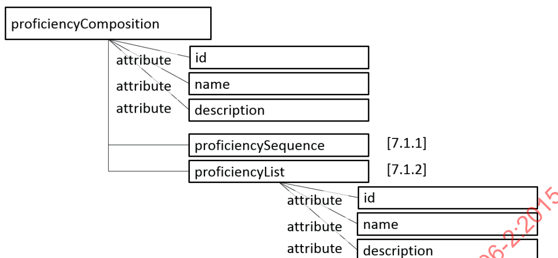
Figure 3 — Proficiency composition model
