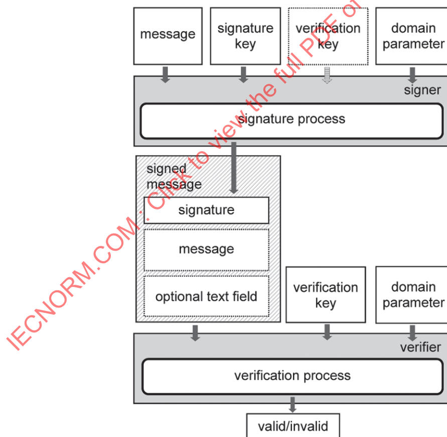
Figure 1 — Signature & verification processes in a conventional signature mechanism
