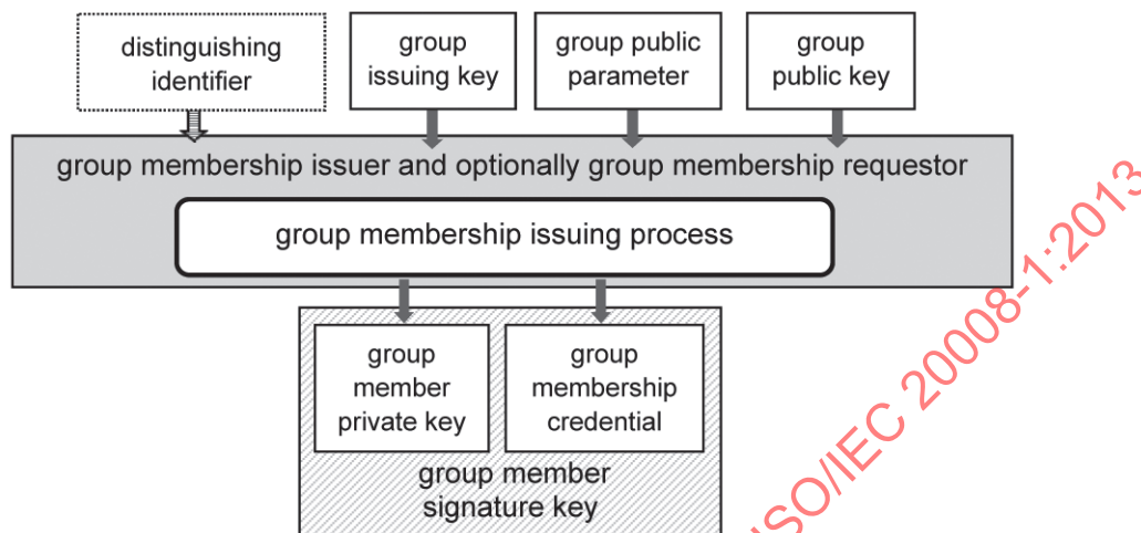
Figure 4 — Group membership issuing process
