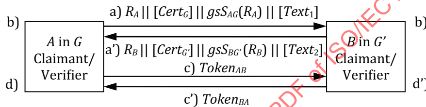
Figure 11 — Two-pass parallel sign-first mutual anonymous authentication
