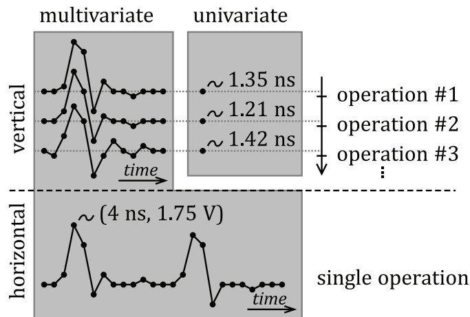
Figure 2 — Illustration of vertical versus horizontal attacks, and multivariate versus univariate side-channel traces
