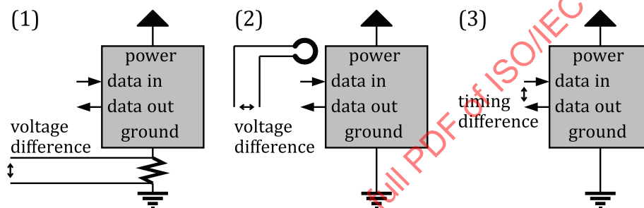
Figure 1 — Three types of side-channels
