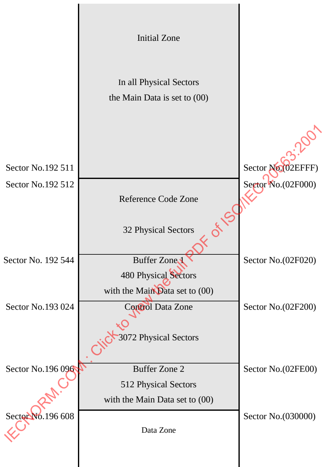
Figure 33 — Lead-in Zone
