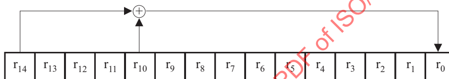
Figure 24 — Feedback shift register for generating scramble data
