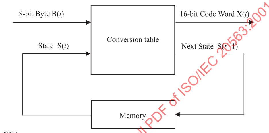
Figure G.1 — Code Words generation
