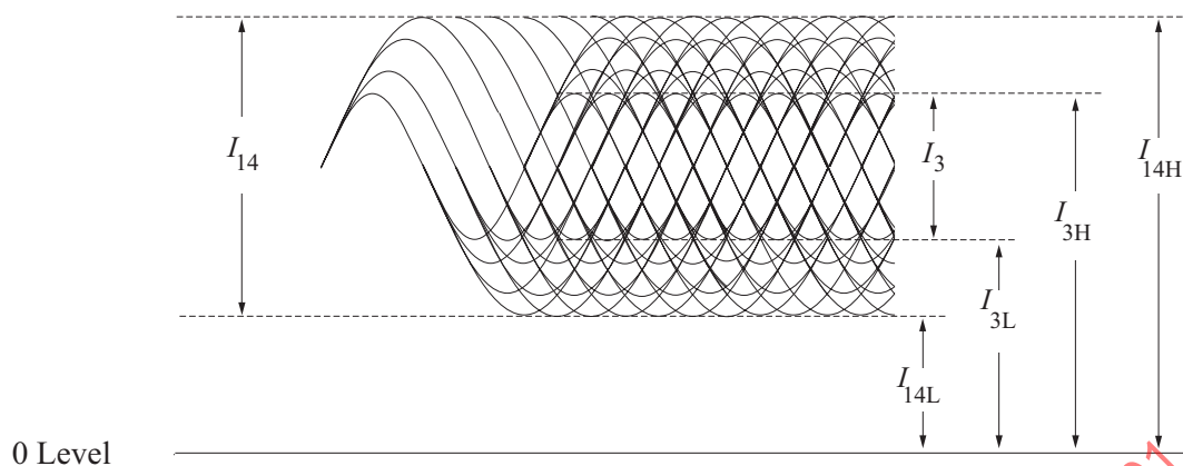
Figure 10 — Modulated amplitude
