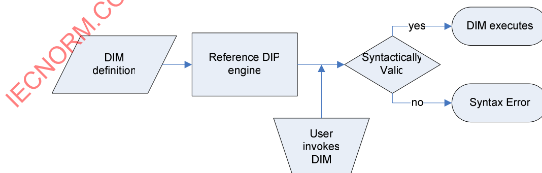
Figure 6 — Testing DIML syntax conformance of a DIM definition
