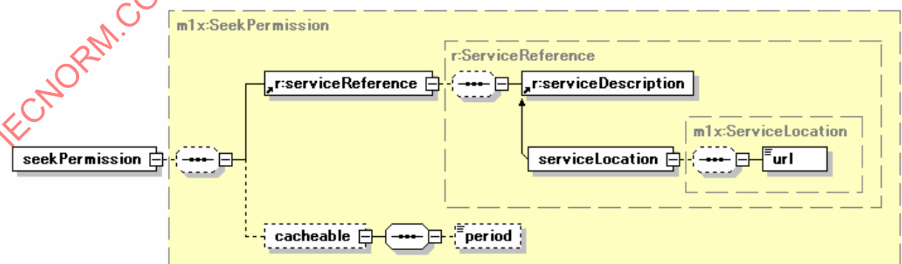
Figure AMD1.13 — m1x:seekPermission Condition
