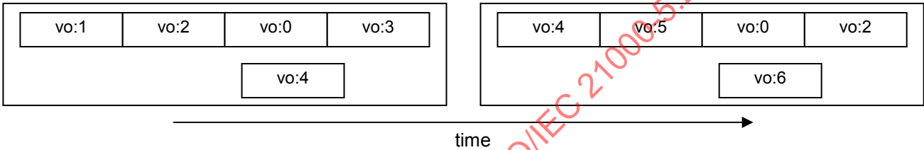
Figure AMD1.9 — Two incorrectly derived Resources
