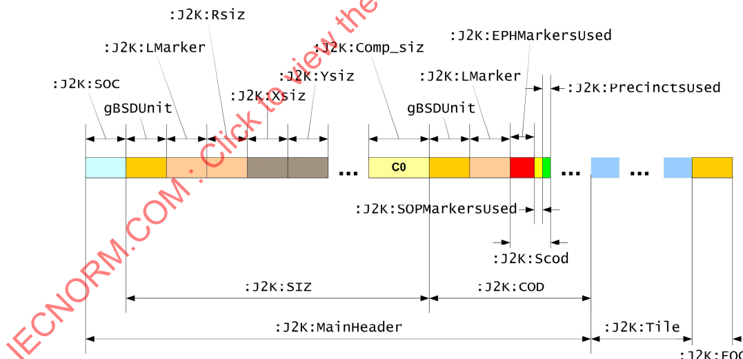
Figure 13 — Example of an adapted/transformed gBS Description for an image
