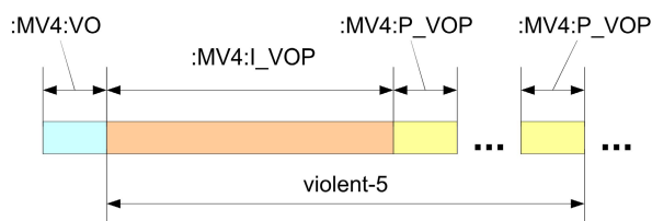
Figure 14 — Example of an original and adapted gBSD for video
