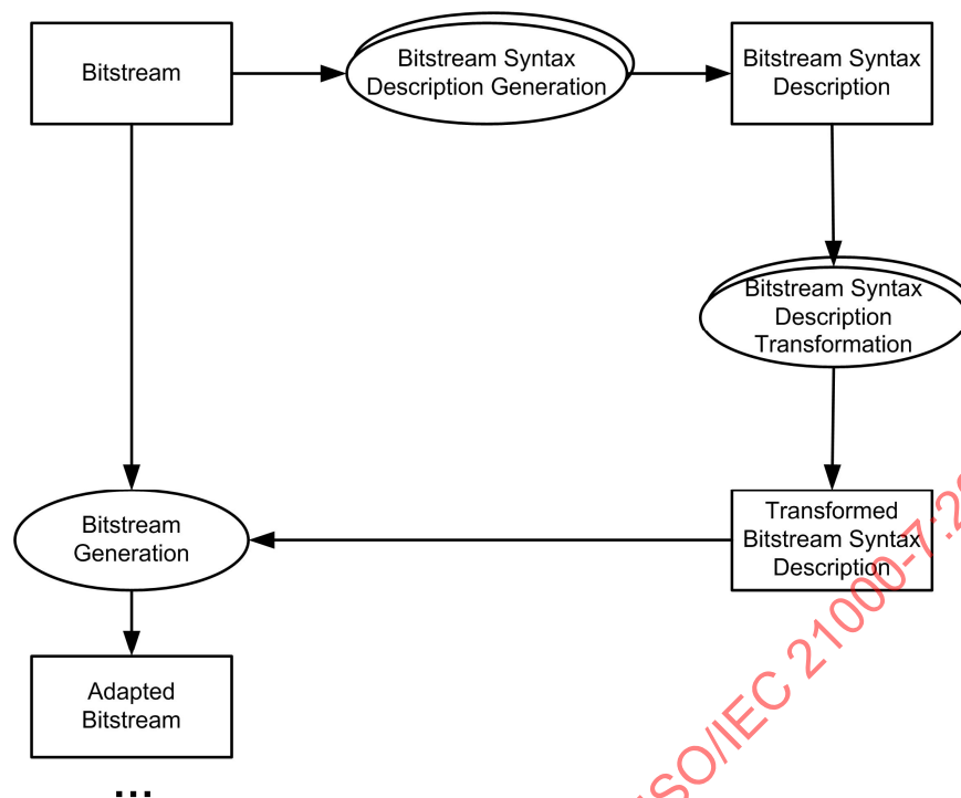
Figure 8 — Adaptation architecture
