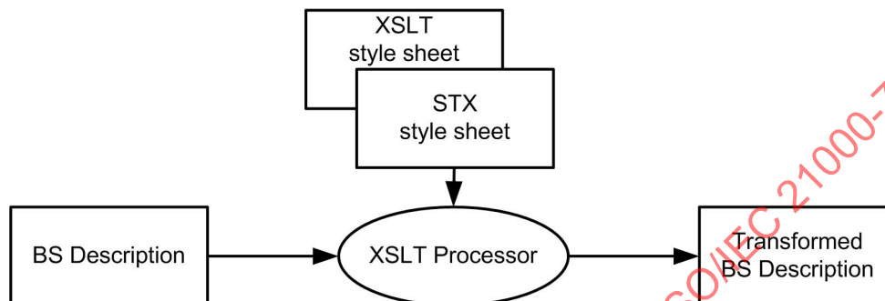
Figure 9 — Architecture of BSD transformation
