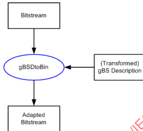
Figure 11 — Architecture of bitstream generation using gBSDtoBin
