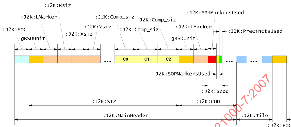
Figure 12 — Example of an original gBS Description for an image
