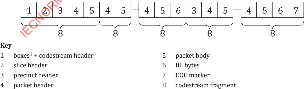
Figure B.1 — Coded codestream fragment
