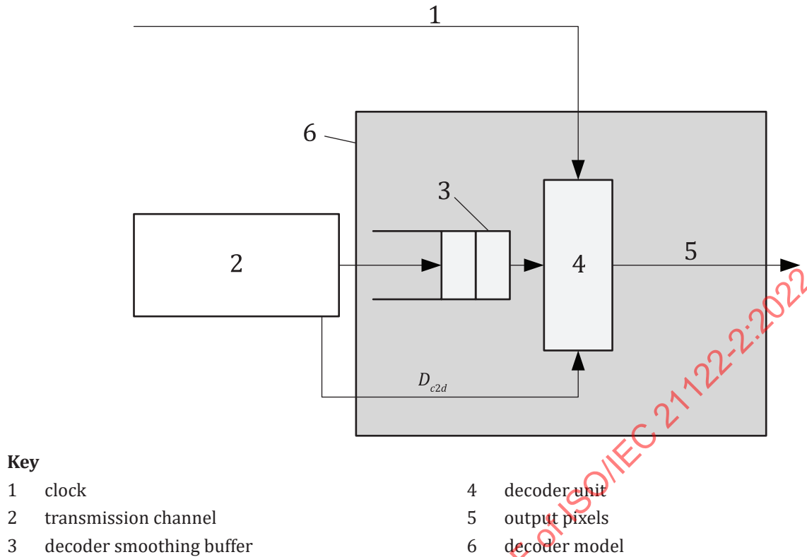
Figure B.4 — JPEG XS decoder model
