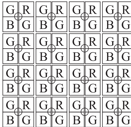
Figure 2 — Example of the interpretation of a GRBG Bayer-type CFA image
