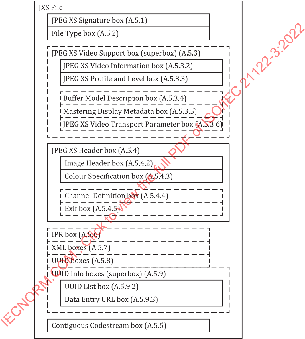
Figure A.1 — Conceptual structure of a JXS file
