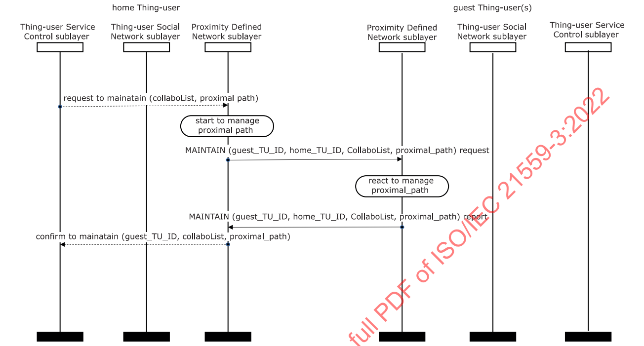
Figure 7 — Sequence chart for proximal path establishment
