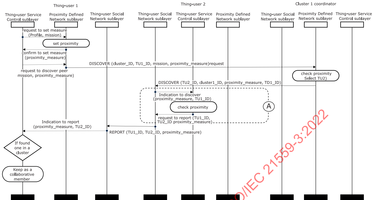
Figure 5 — Sequence chart for thing-user discovery in case no appropriate thing-user was found
