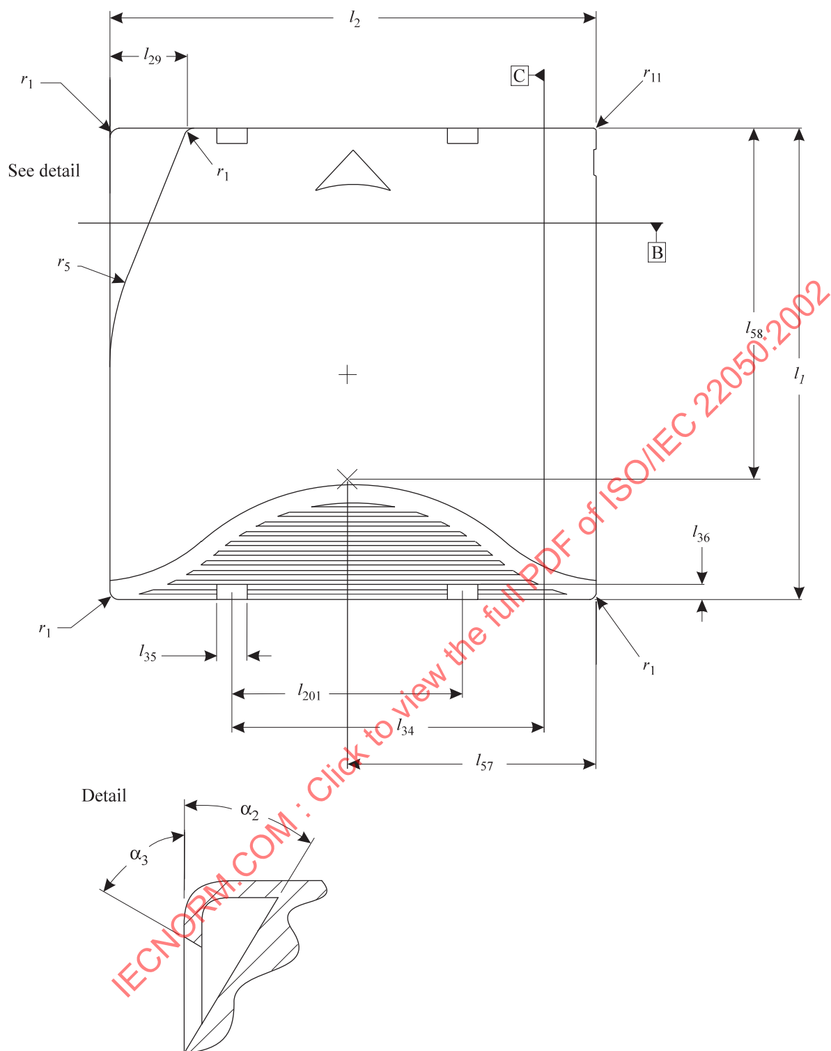
Figure 4 - Top side
