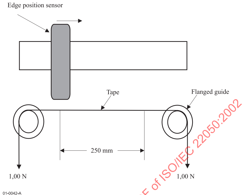
Figure 20 - Measurement of edge deviation
