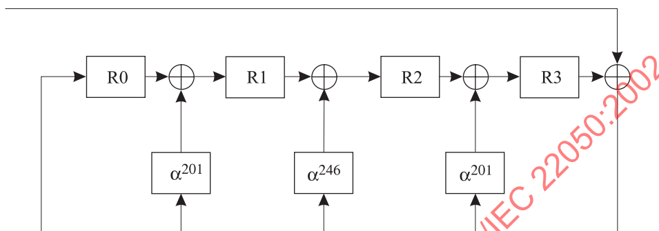
Figure 32 - CRC generator circuit
