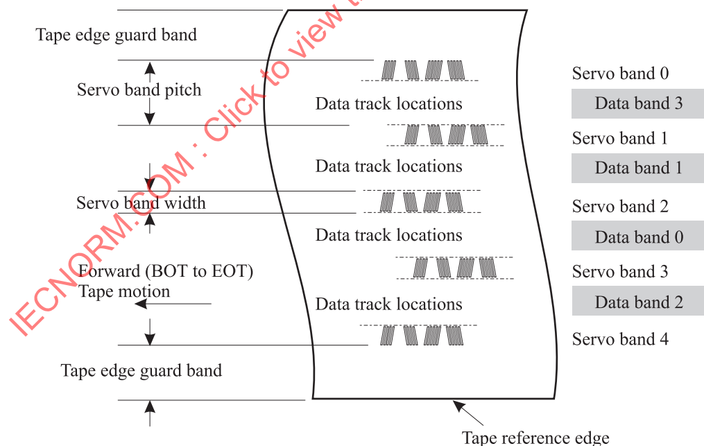
Figure 25 – Servo band locations
