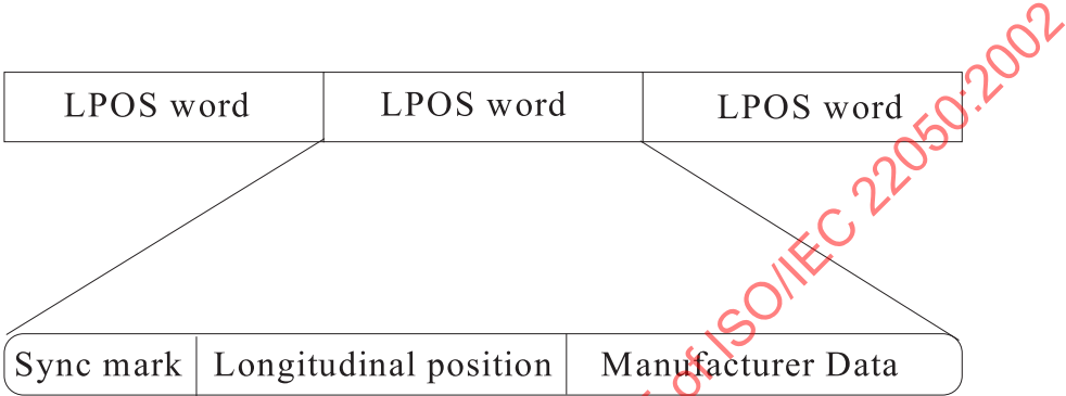
Figure 29 LPOS word layout
