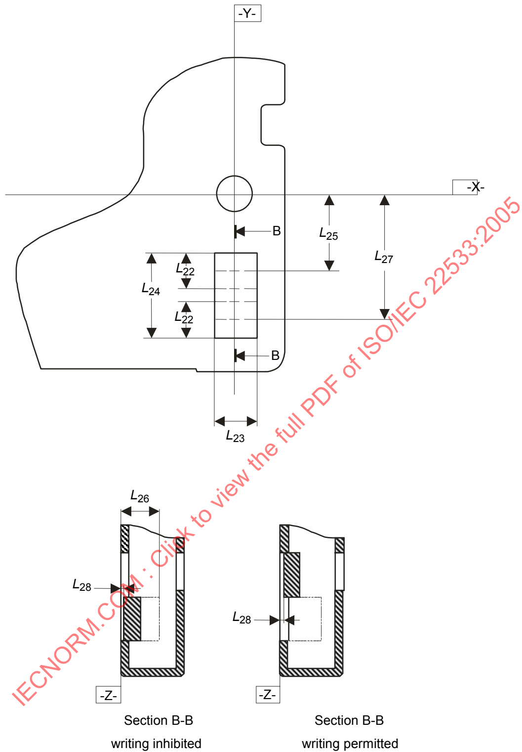
Figure 6 – Functional Areas FA1 and FA2, seen on Side A and in cross-section
